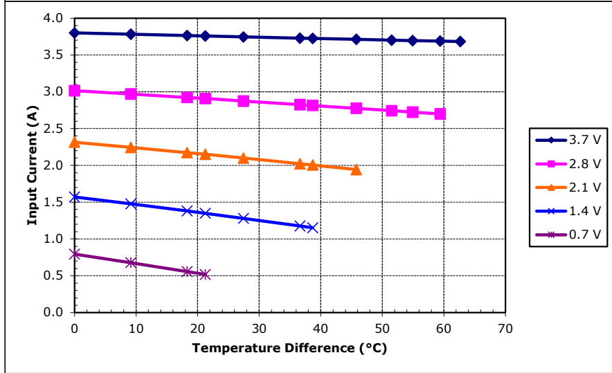
Potted VT-31-1.0-1.3 at a hot-side temperature of 30 °C
