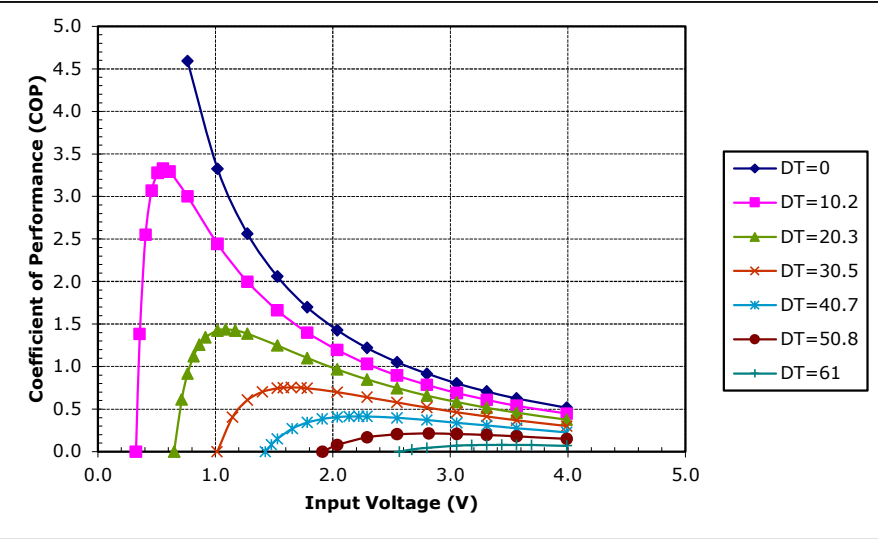
Potted VT-31-1.0-1.3 at a hot-side temperature of 50 °C
