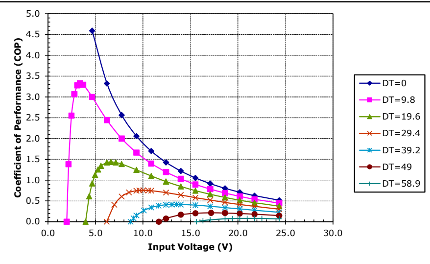
Unpotted VT-199-1.4-1.15 at a hot-side temperature of 30 °C
