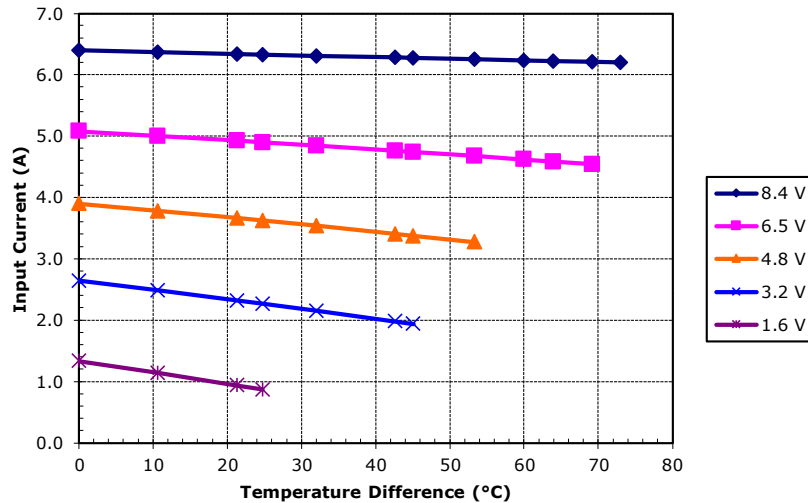
Potted TE-63-1.4-1.5 at a hot-side temperature of 50 °C
