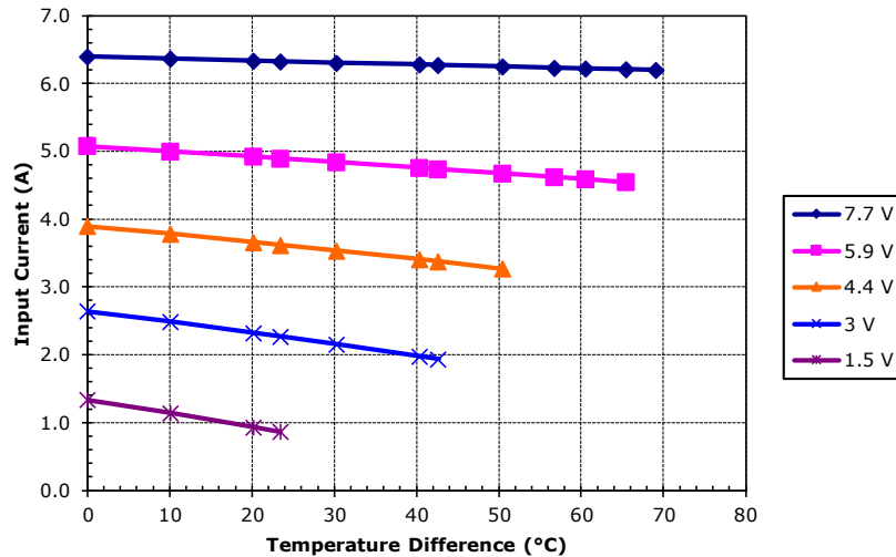
Unpotted TE-63-1.4-1.5 at a hot-side temperature of 30 °C
