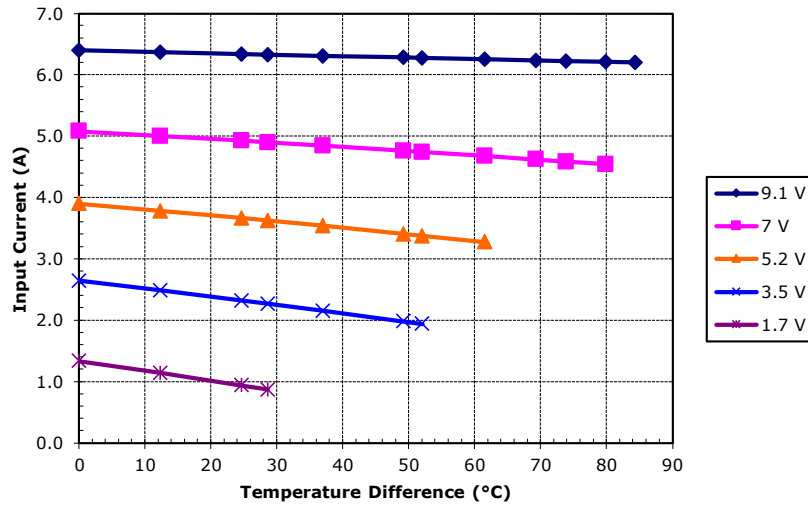
Unpotted TE-63-1.4-1.5 at a hot-side temperature of 70 °C
