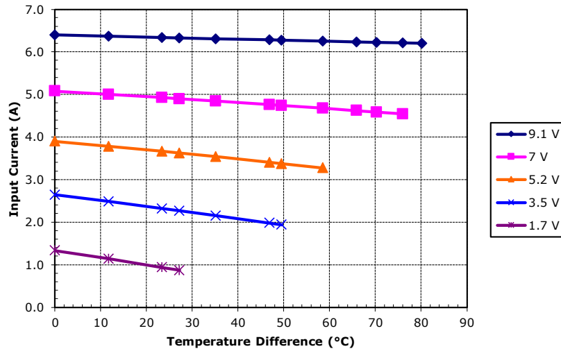
Potted TE-63-1.4-1.5 at a hot-side temperature of 70 °C
