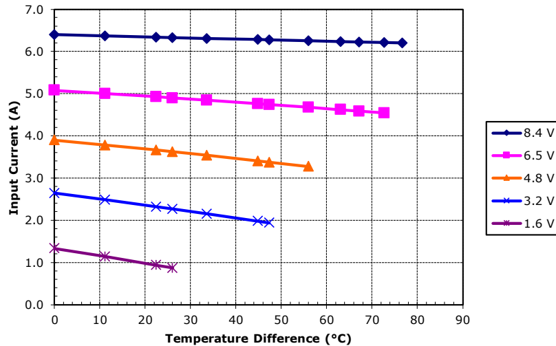
Unpotted TE-63-1.4-1.5 at a hot-side temperature of 50 °C
