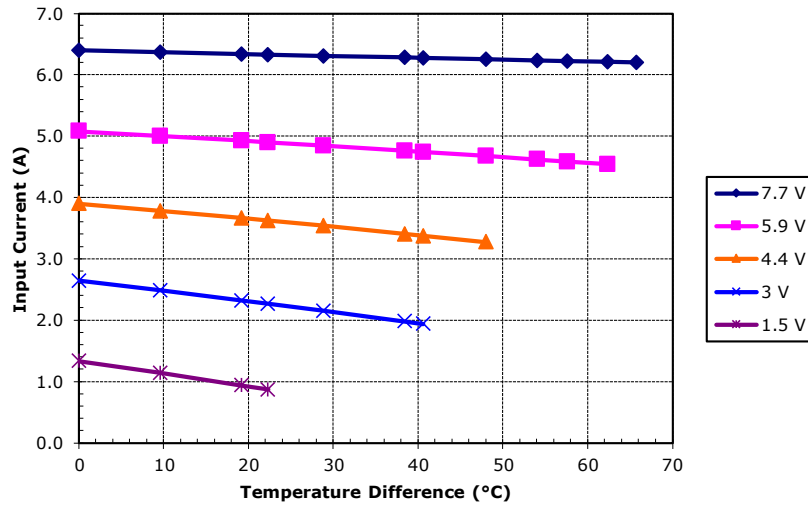
Potted TE-63-1.4-1.5 at a hot-side temperature of 30 °C
