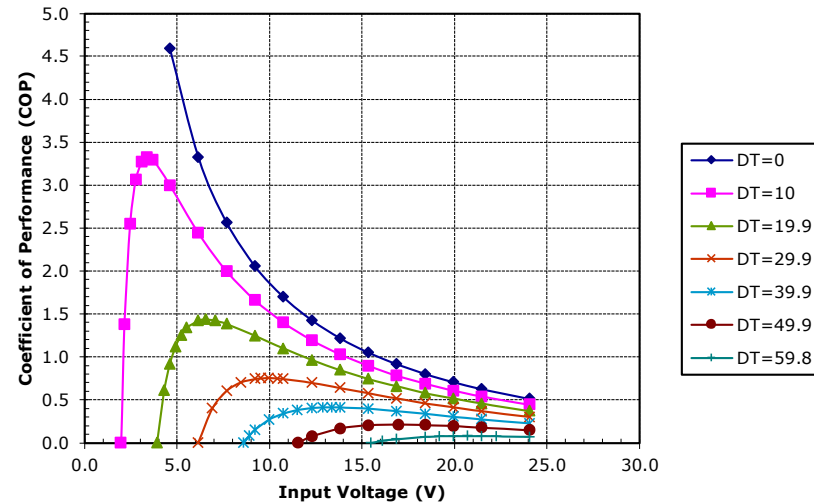
Potted HP-199-1.4-1.5 at a hot-side temperature of 30 °C
