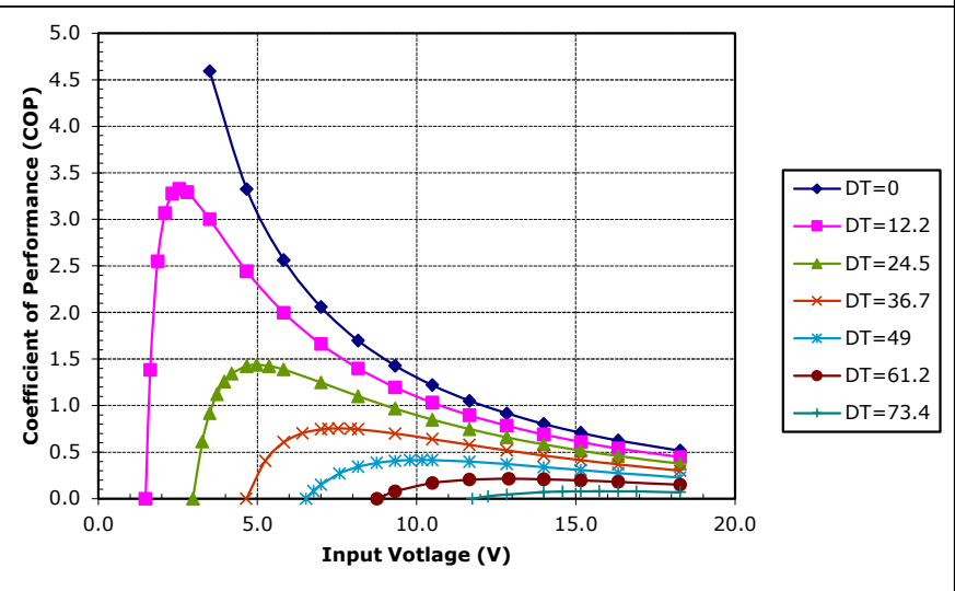
Unpotted HP-127-1.0-1.3-71 at a hot-side temperature of 70 °C
