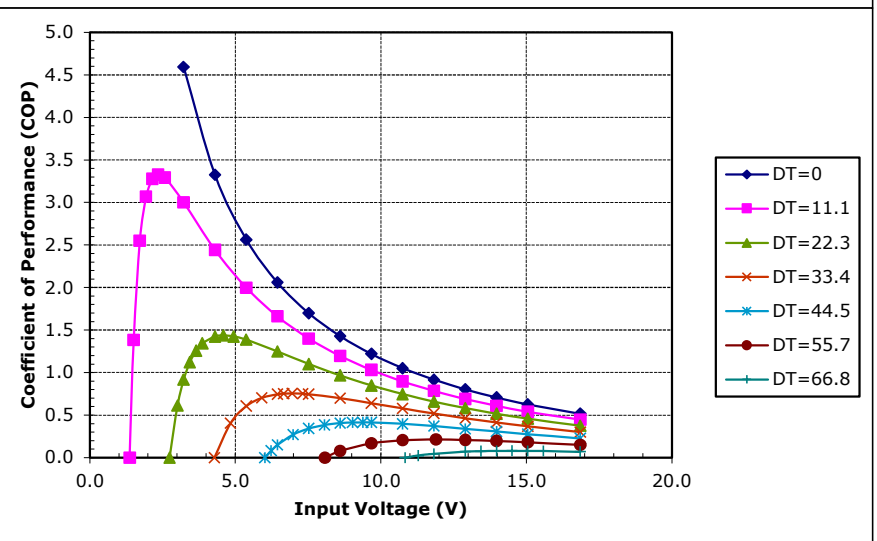
Unpotted HP-127-1.0-1.3-71 at a hot-side temperature of 50 °C
