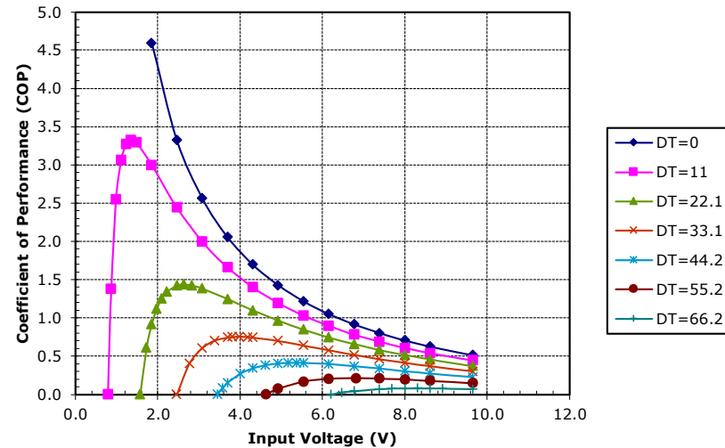
Unpotted TE-71-1.0-1.3 at a hot-side temperature of 50 °C
