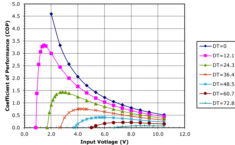
Unpotted TE-71-1.0-1.3 at a hot-side temperature of 70 °C
