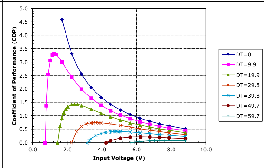
Unpotted TE-71-1.0-1.3 at a hot-side temperature of 30 °C
