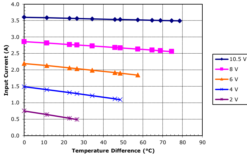
Potted TE-71-1.0-1.3 at a hot-side temperature of 70 °C
