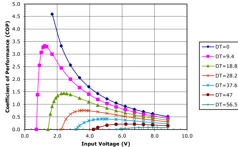
Potted TE-71-1.0-1.3 at a hot-side temperature of 30 °C
