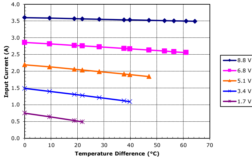
Potted TE-71-1.0-1.3 at a hot-side temperature of 30 °C
