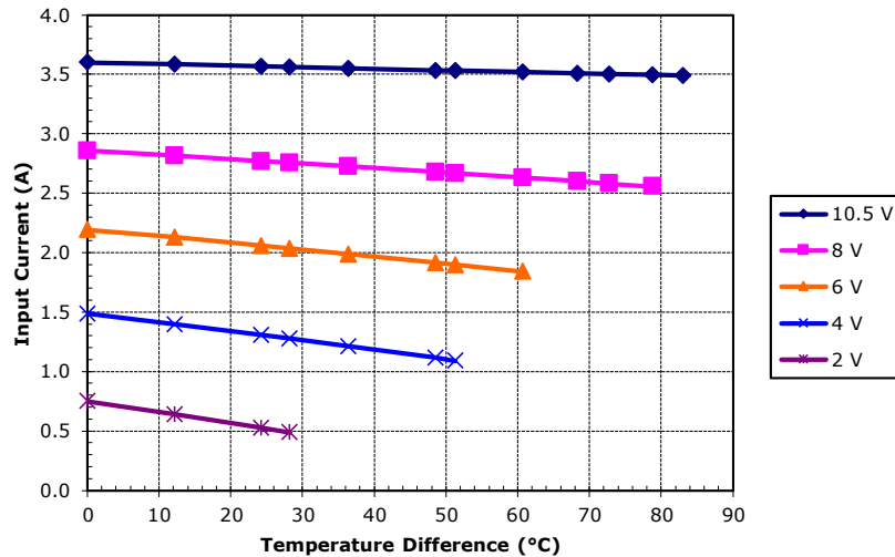
Unpotted TE-71-1.0-1.3 at a hot-side temperature of 70 °C
