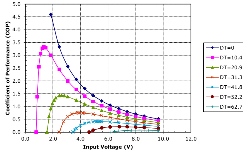
Potted TE-71-1.0-1.3 at a hot-side temperature of 50 °C
