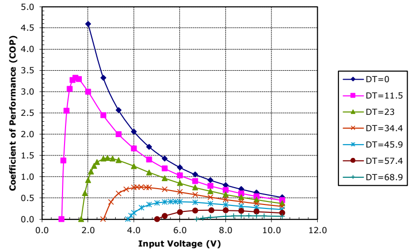
Potted TE-71-1.0-1.3 at a hot-side temperature of 70 °C
