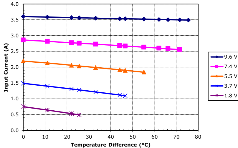
Unpotted TE-71-1.0-1.3 at a hot-side temperature of 50 °C
