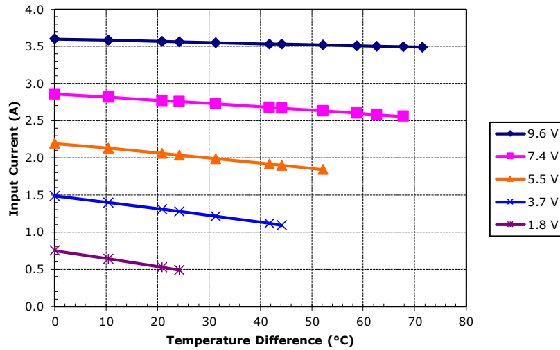
Potted TE-71-1.0-1.3 at a hot-side temperature of 50 °C
