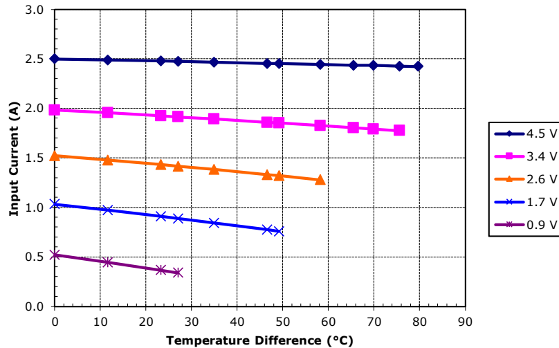
Potted TE-31-1.0-2.0 at a hot-side temperature of 70 °C
