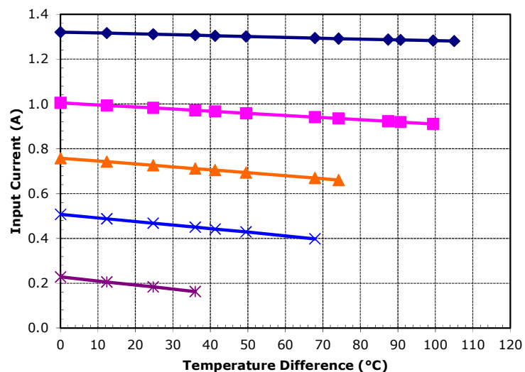
Potted TE-2-(31-12)-1.0 at a hot-side temperature of 70 °C
