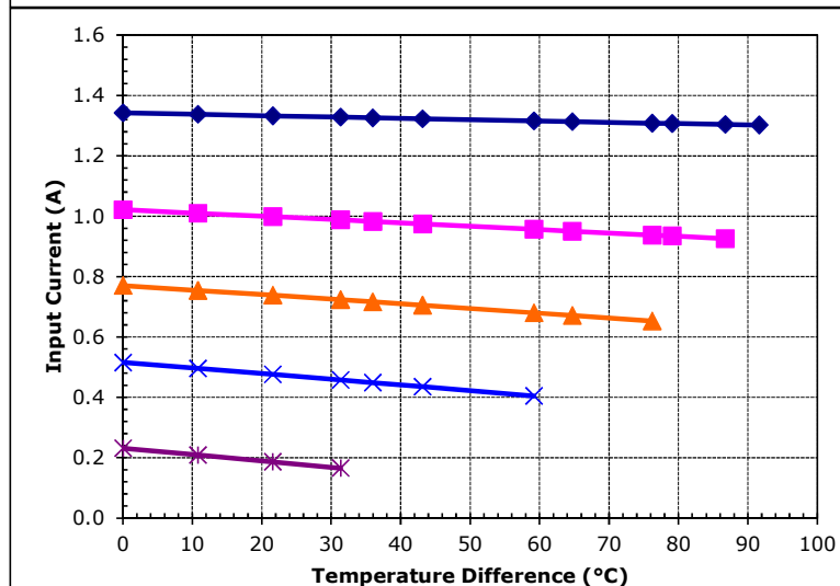
Unpotted TE-2-(31-12)-1.0 at a hot-side temperature of 30 °C
