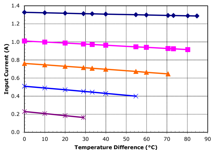
Potted TE-2-(31-12)-1.0 at a hot-side temperature of 30 °C
