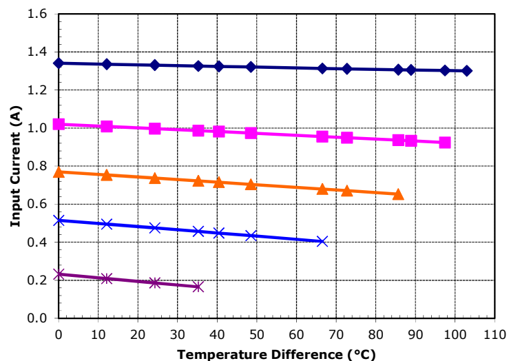
Unpotted TE-2-(31-12)-1.0 at a hot-side temperature of 50 °C
