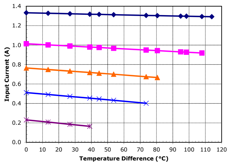
Unpotted TE-2-(31-12)-1.0 at a hot-side temperature of 70 °C
