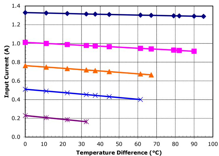
Potted TE-2-(31-12)-1.0 at a hot-side temperature of 50 °C
