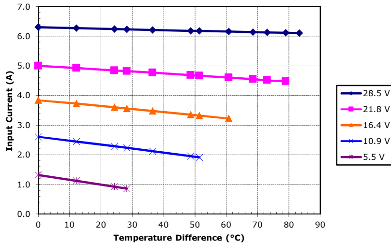
Potted VT-199-1.4-1.5 at a hot-side temperature of 70 °C
