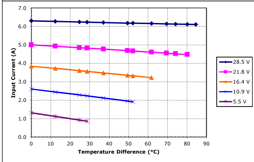
Unpotted VT-199-1.4-1.5 at a hot-side temperature of 70 °C
