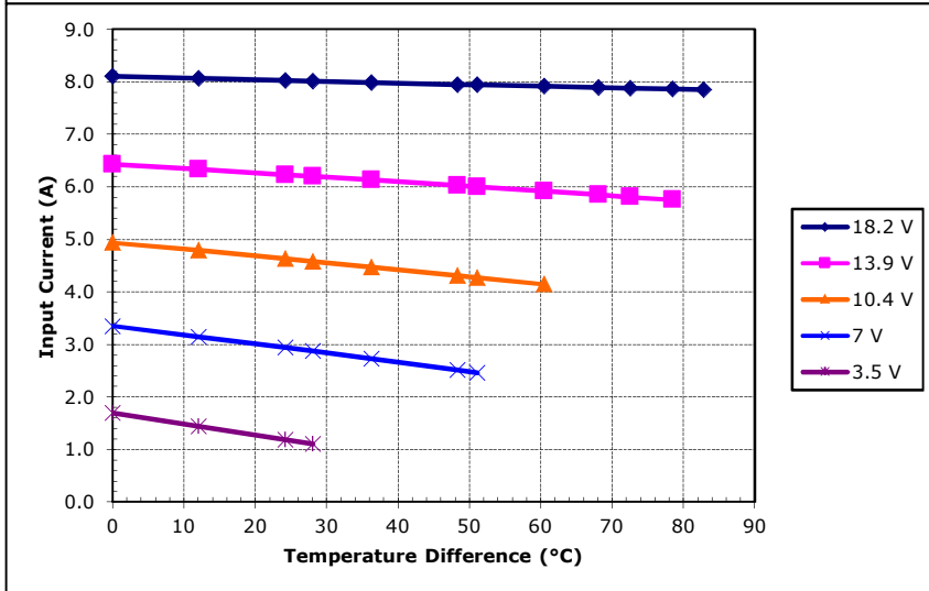
Unpotted VT-127-1.4-1.15-71 at a hot-side temperature of 70 °C
