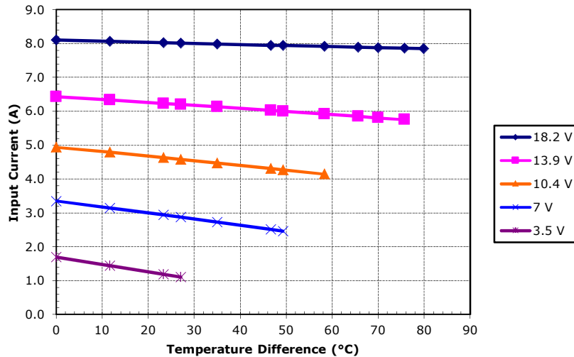
Potted VT-127-1.4-1.15-71 at a hot-side temperature of 70 °C
