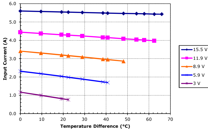
Unpotted HP-127-1.0-0.8 at a hot-side temperature of 30 °C
