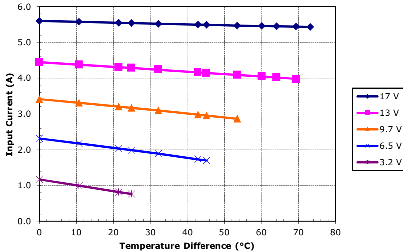
Unpotted HP-127-1.0-0.8 at a hot-side temperature of 50 °C
