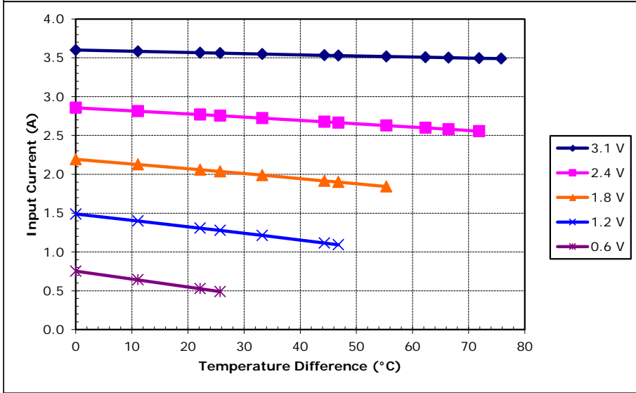
Unpotted TE-23-1.0-1.3 at a hot-side temperature of 50 °C
