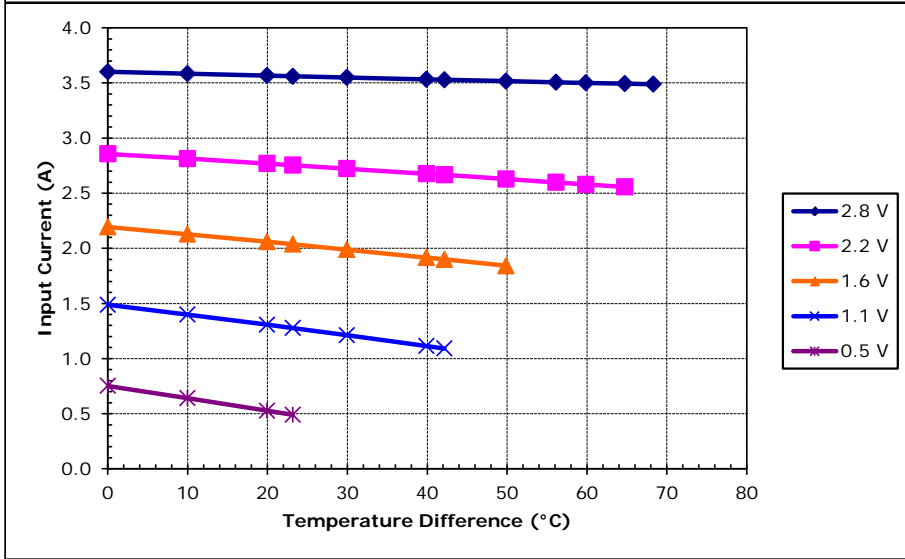
Unpotted TE-23-1.0-1.3 at a hot-side temperature of 30 °C
