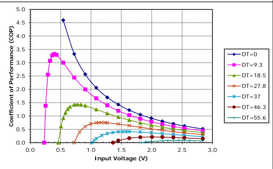
Potted TE-23-1.0-1.3 at a hot-side temperature of 30 °C
