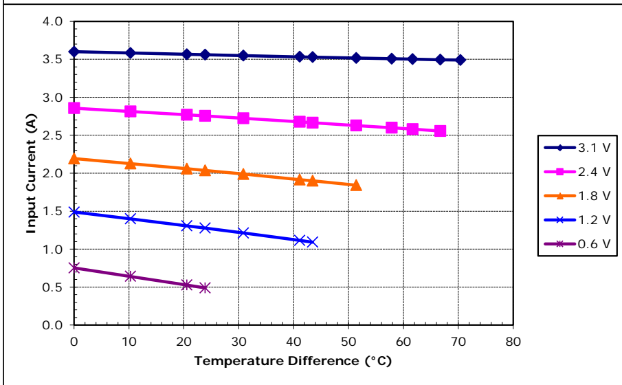
Potted TE-23-1.0-1.3 at a hot-side temperature of 50 °C
