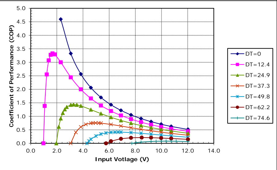
Unpotted TE-83-1.0-1.5 at a hot-side temperature of 70 °C
