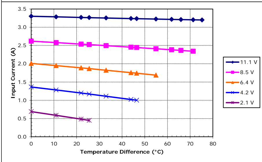
Potted TE-83-1.0-1.5 at a hot-side temperature of 50 °C
