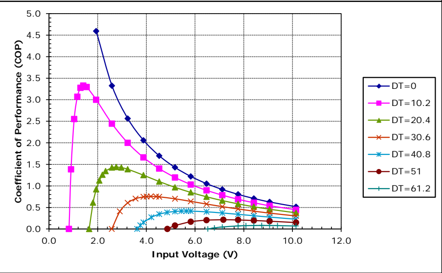
Unpotted TE-83-1.0-1.5 at a hot-side temperature of 30 °C
