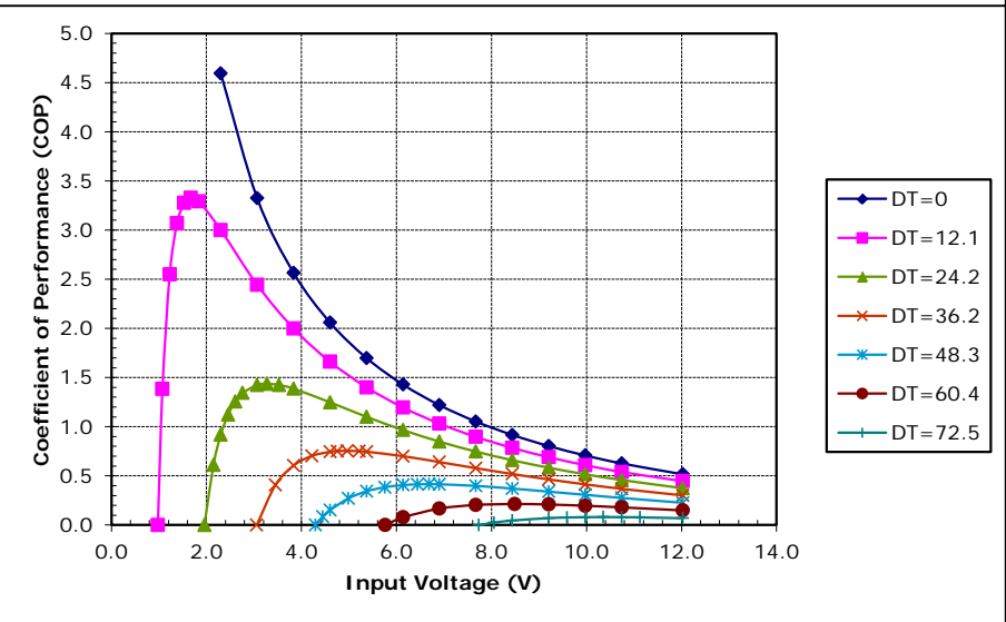
Potted TE-83-1.0-1.5 at a hot-side temperature of 70 °C
