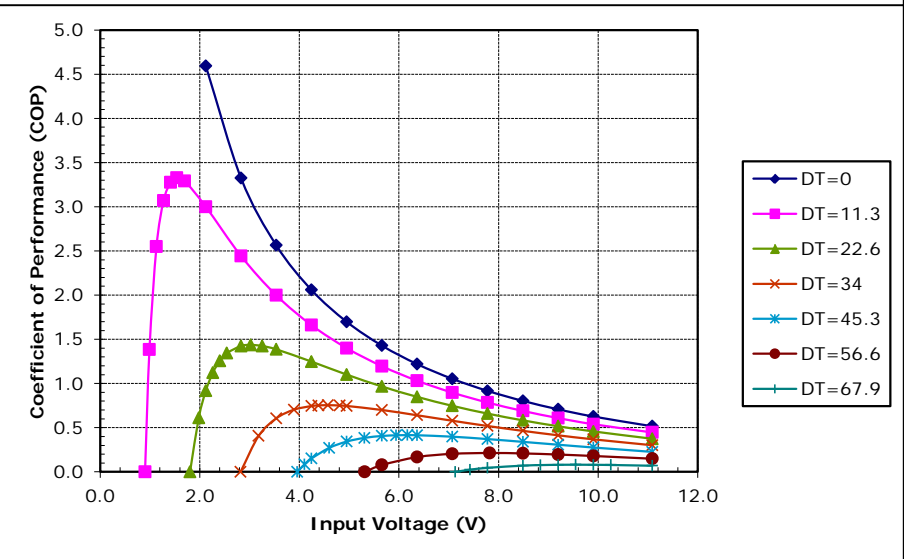
Unpotted TE-83-1.0-1.5 at a hot-side temperature of 50 °C
