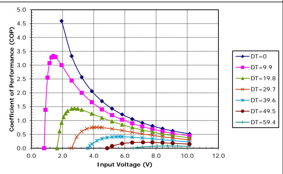
Potted TE-83-1.0-1.5 at a hot-side temperature of 30 °C
