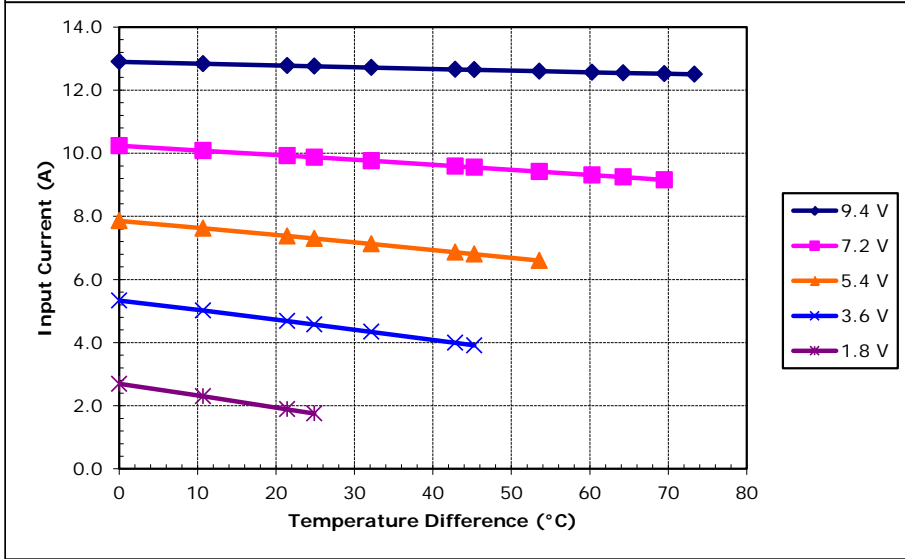
Potted TE-71-2.0-1.5 at a hot-side temperature of 50 °C
