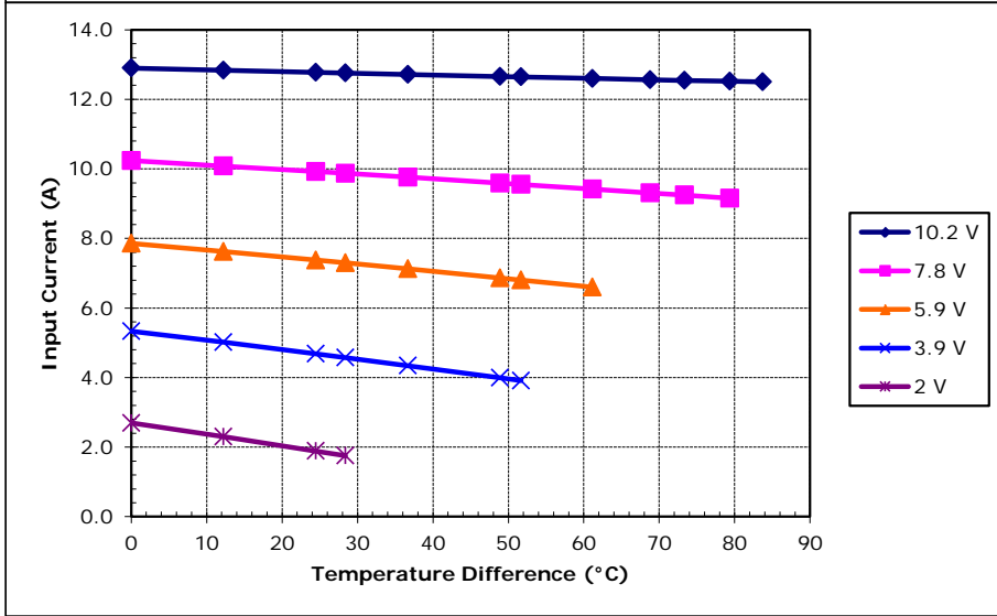
Unpotted TE-71-2.0-1.5 at a hot-side temperature of 70 °C
