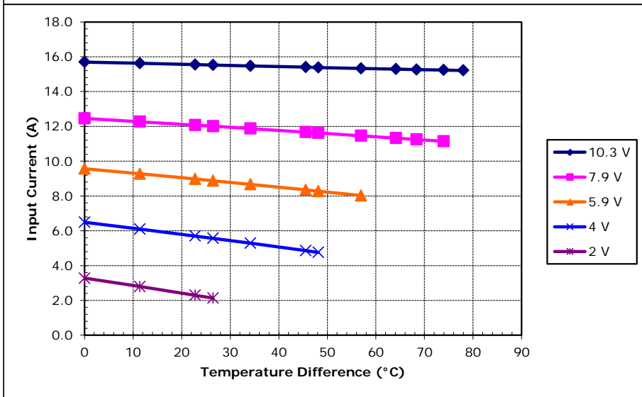
Potted TE-71-2.0-1.15 at a hot-side temperature of 70 °C
