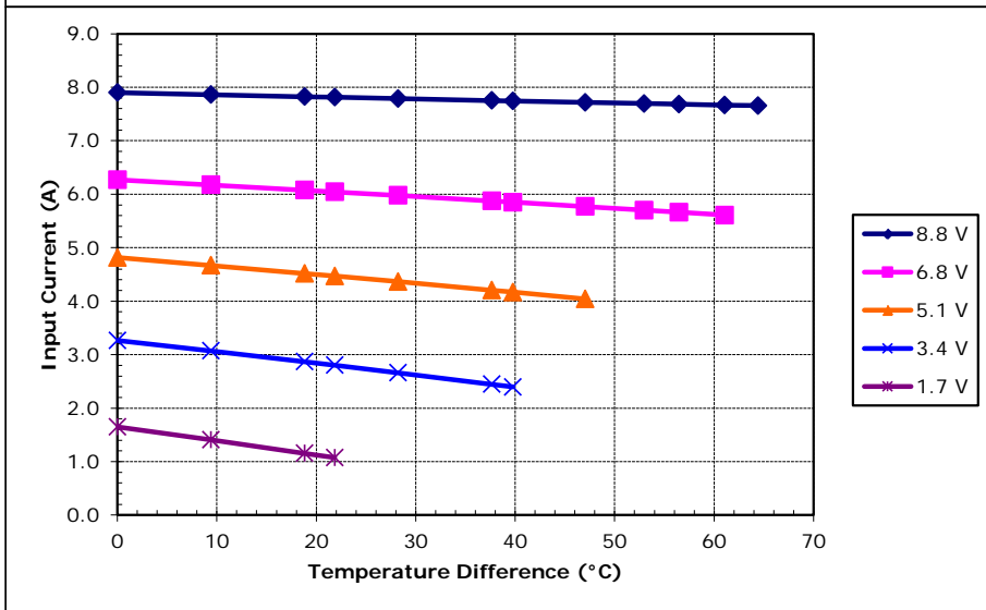
Potted TE-71-1.4-1.15 at a hot-side temperature of 30 °C
