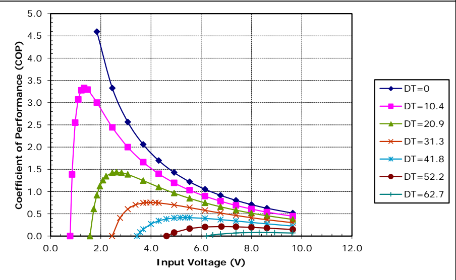
Potted TE-71-1.4-1.15 at a hot-side temperature of 50 °C
