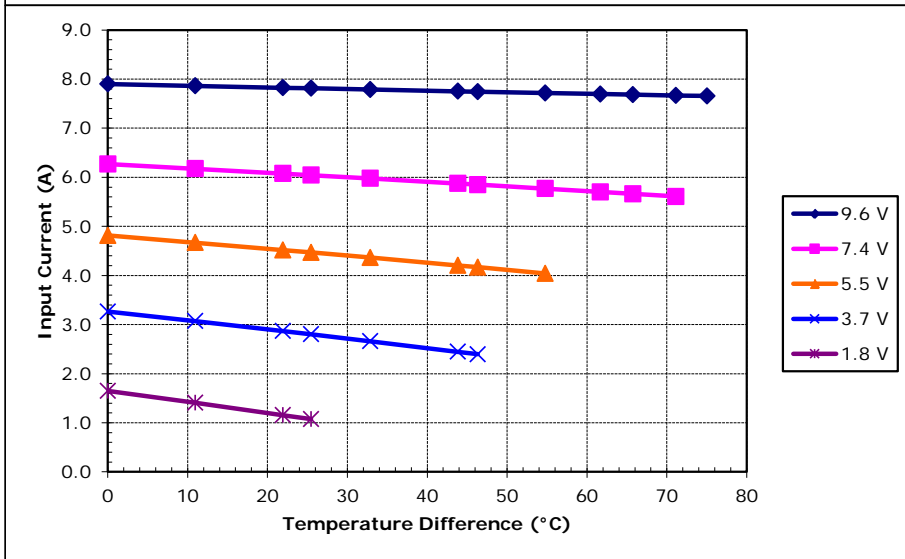
Unpotted TE-71-1.4-1.15 at a hot-side temperature of 50 °C
