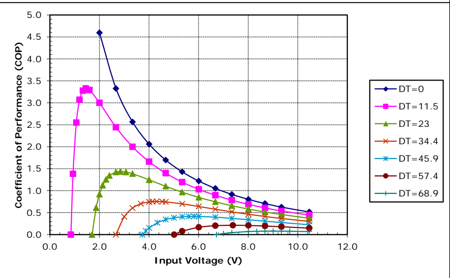
Potted TE-71-1.4-1.15 at a hot-side temperature of 70 °C
