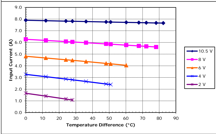
Unpotted TE-71-1.4-1.15 at a hot-side temperature of 70 °C
