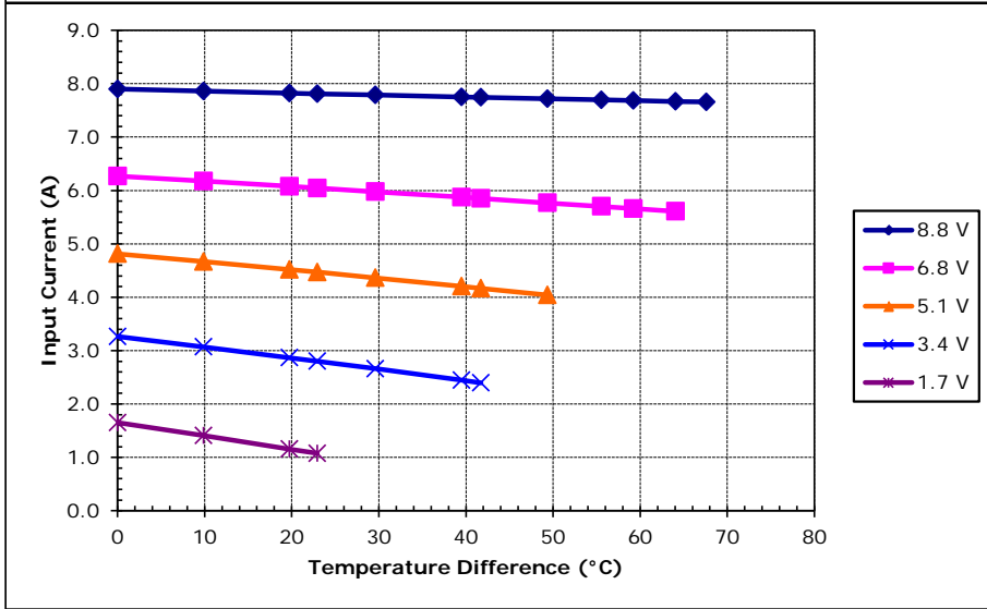
Unpotted TE-71-1.4-1.15 at a hot-side temperature of 30 °C
