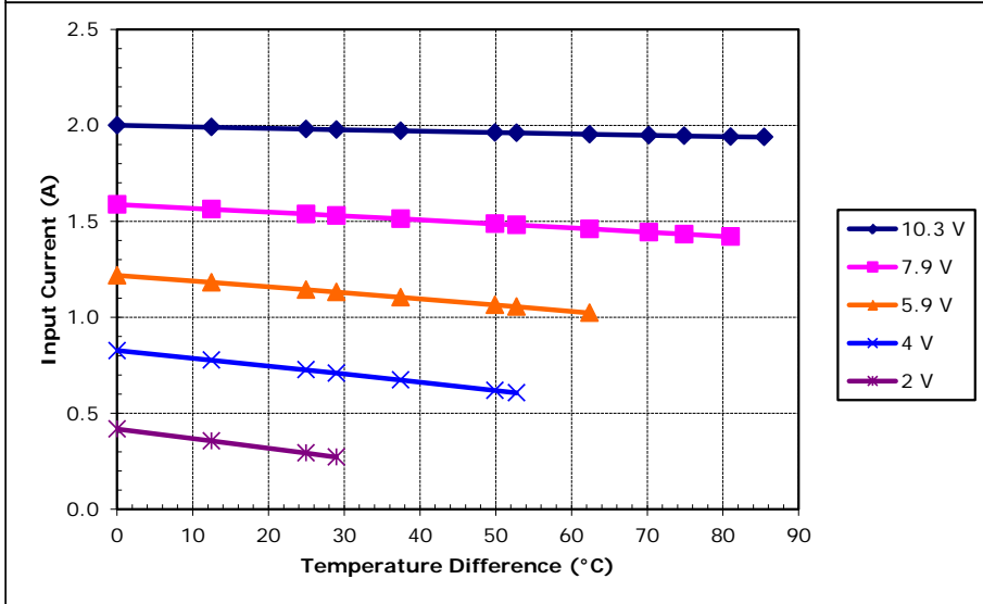
Unpotted TE-71-1.0-2.5 at a hot-side temperature of 70 °C
