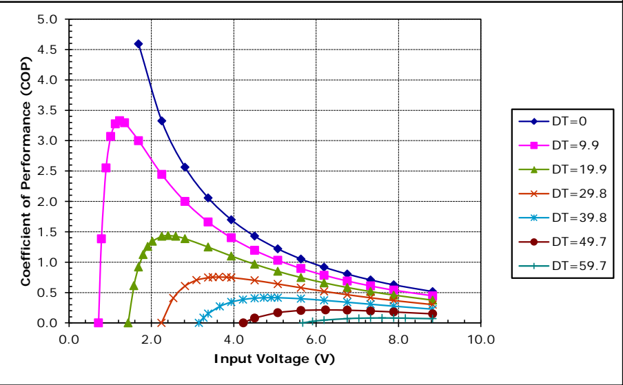
Unpotted TE-71-1.0-1.3 at a hot-side temperature of 30 °C
