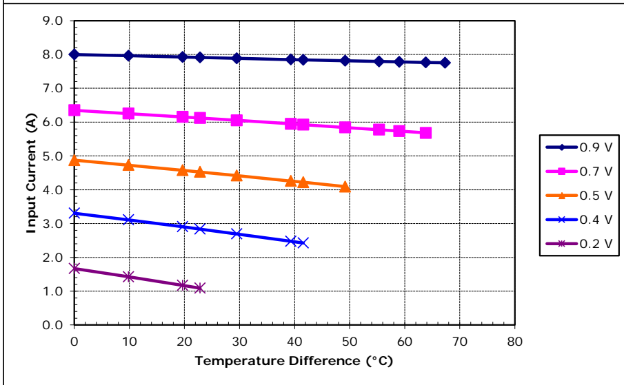
Potted TE-7-2.0-2.5 at a hot-side temperature of 50 °C
