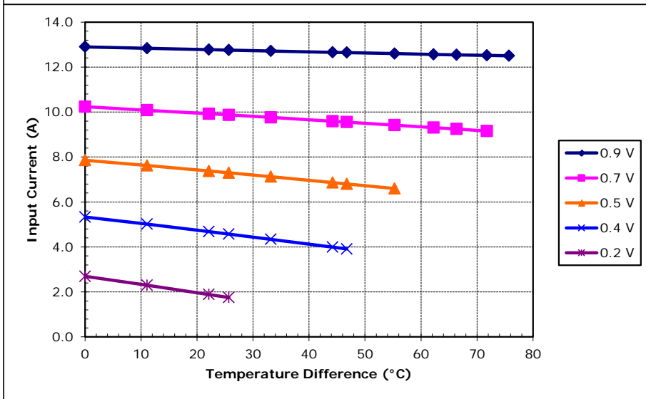
Unpotted TE-7-2.0-1.5 at a hot-side temperature of 50 °C
