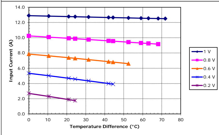
Potted TE-7-2.0-1.5 at a hot-side temperature of 70 °C
