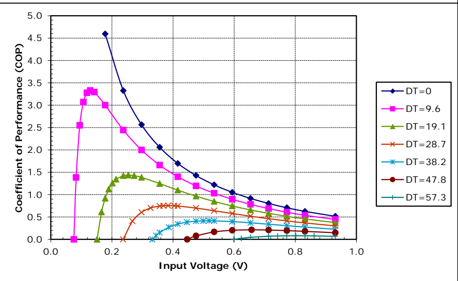
Potted TE-7-2.0-1.5 at a hot-side temperature of 50 °C
