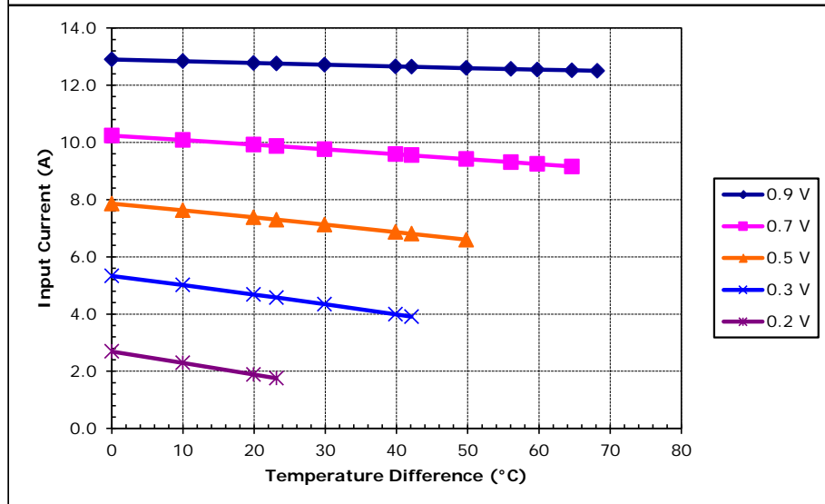
Unpotted TE-7-2.0-1.5 at a hot-side temperature of 30 °C
