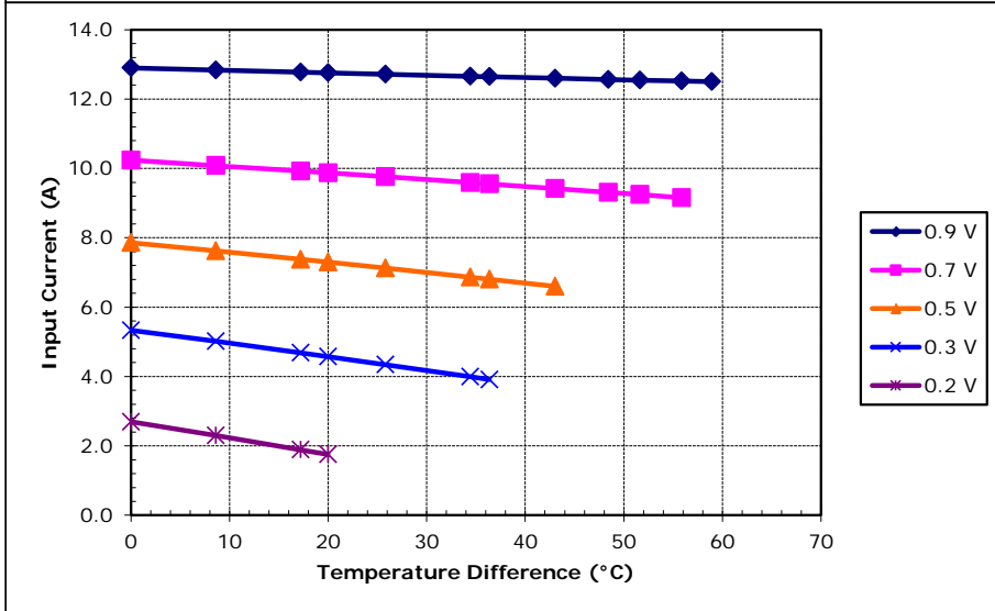
Potted TE-7-2.0-1.5 at a hot-side temperature of 30 °C
