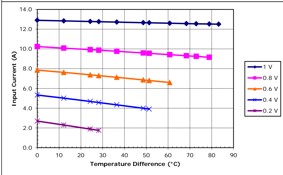
Unpotted TE-7-2.0-1.5 at a hot-side temperature of 70 °C
