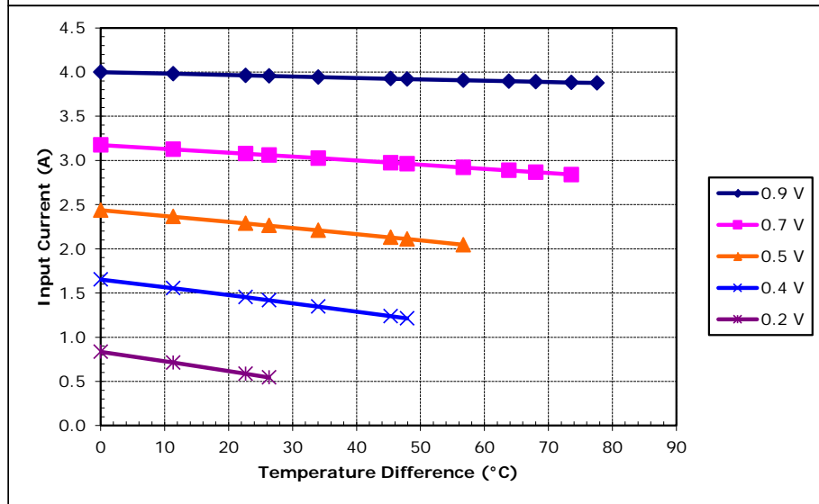
Unpotted TE-7-1.4-2.5 at a hot-side temperature of 50 °C
