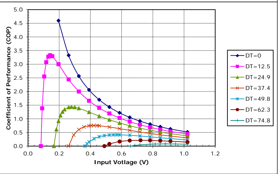
Unpotted TE-7-1.4-2.5 at a hot-side temperature of 70 °C
