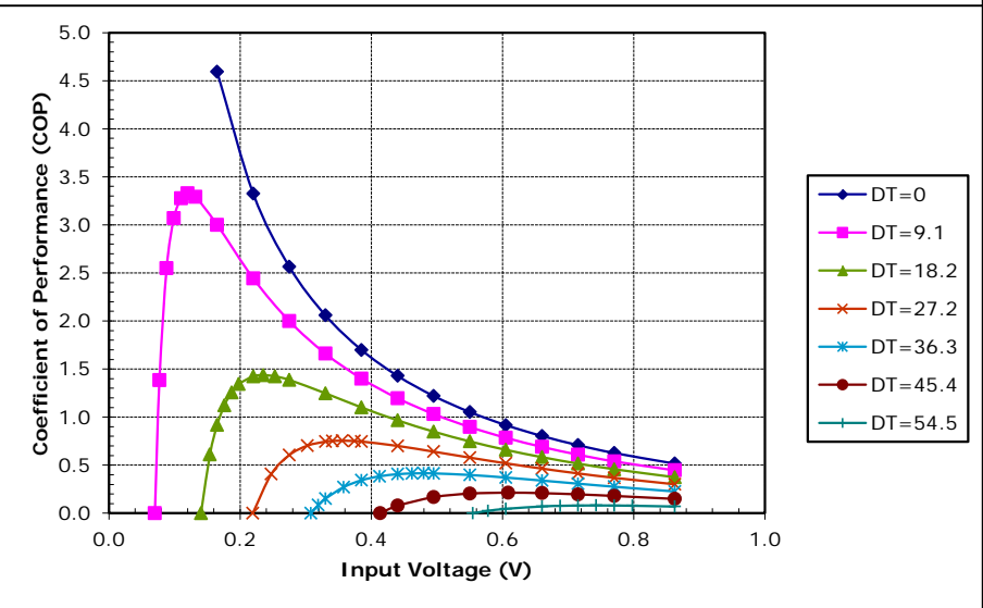
Potted TE-7-1.4-2.5 at a hot-side temperature of 30 °C
