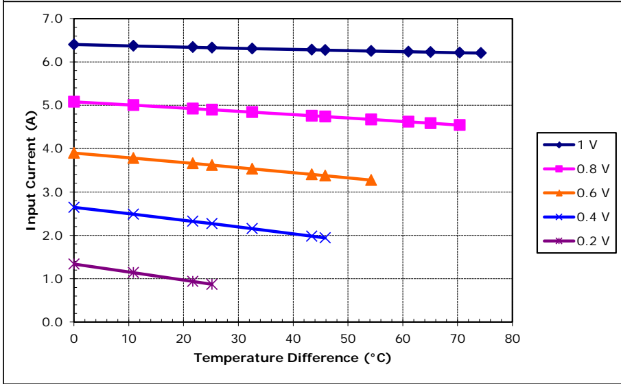
Potted TE-7-1.4-1.5 at a hot-side temperature of 70 °C
