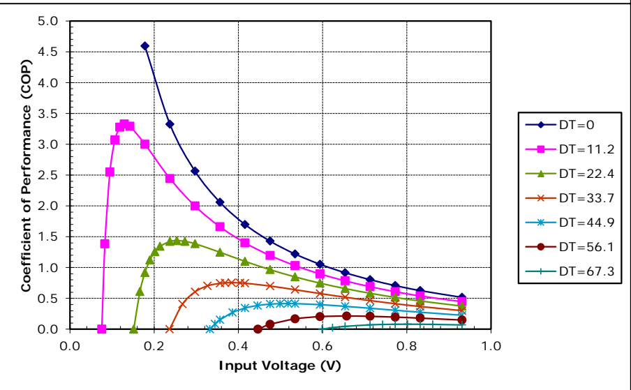
Unpotted TE-7-1.4-1.5 at a hot-side temperature of 50 °C
