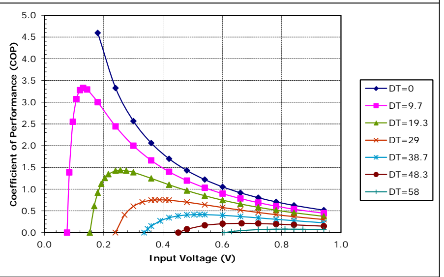
Potted TE-7-1.0-2.5 at a hot-side temperature of 50 °C
