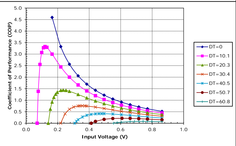
Unpotted TE-7-1.0-2.5 at a hot-side temperature of 30 °C
