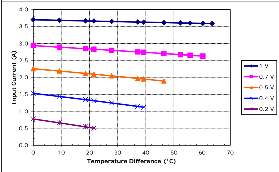
Potted TE-7-1.0-1.3 at a hot-side temperature of 50 °C
