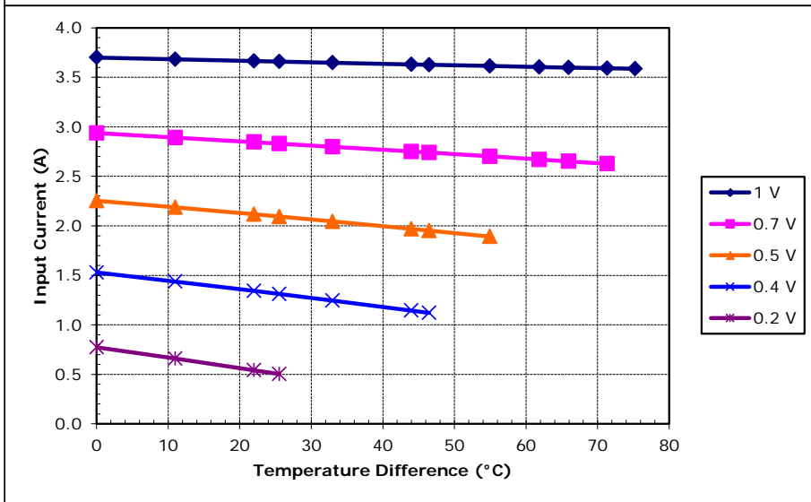
Unpotted TE-7-1.0-1.3 at a hot-side temperature of 50 °C
