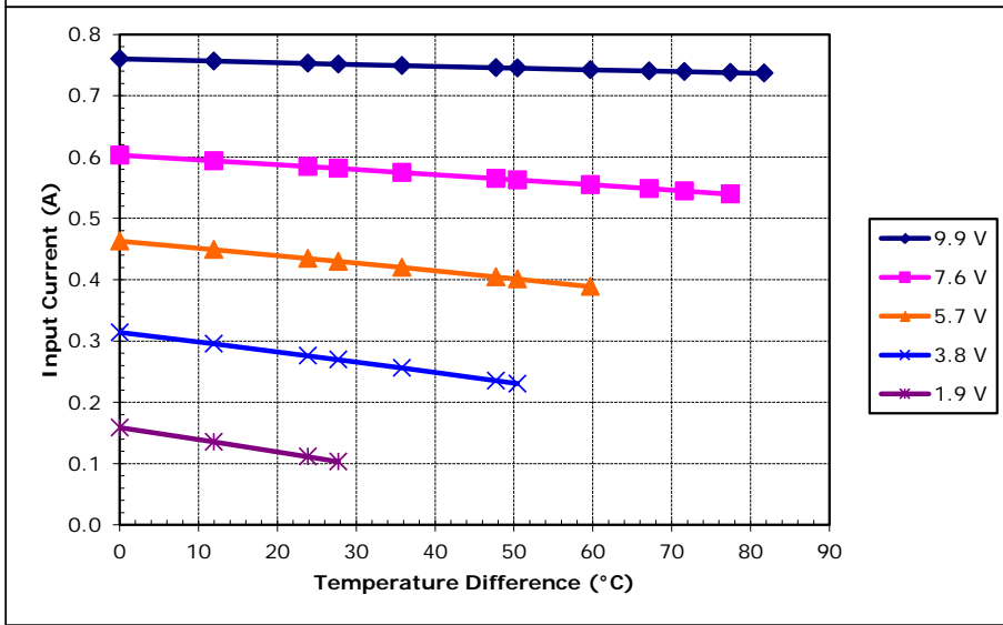
Potted TE-66-0.45-1.3 at a hot-side temperature of 70 °C
