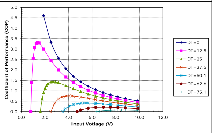
Unpotted TE-66-0.45-1.3 at a hot-side temperature of 70 °C
