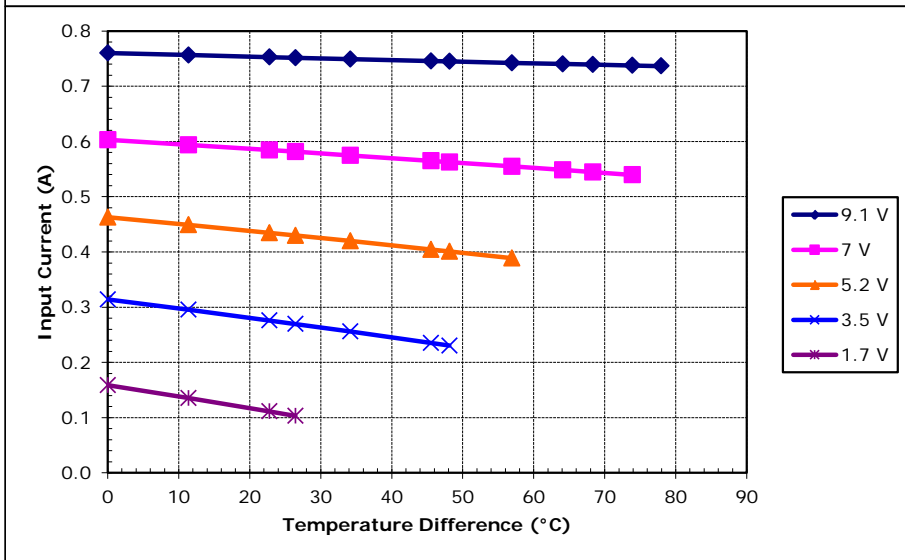
Unpotted TE-66-0.45-1.3 at a hot-side temperature of 50 °C
