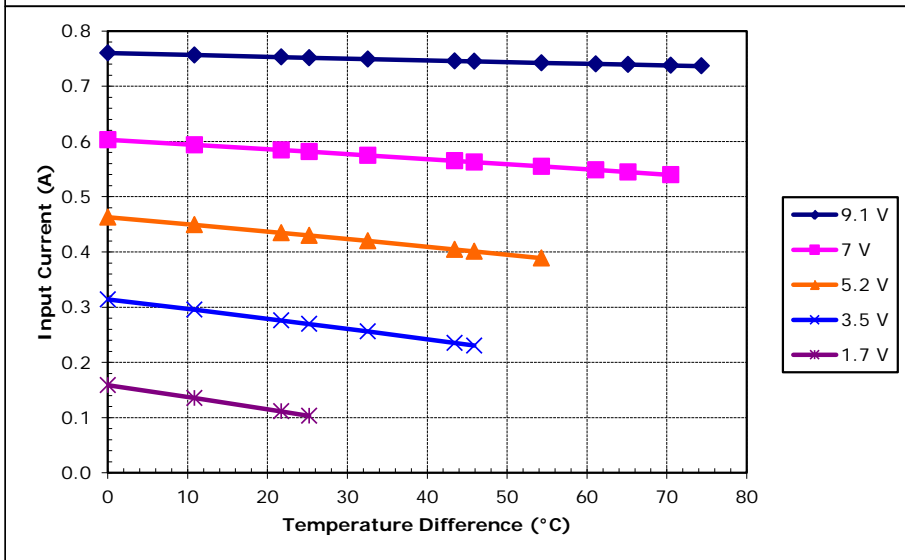
Potted TE-66-0.45-1.3 at a hot-side temperature of 50 °C
