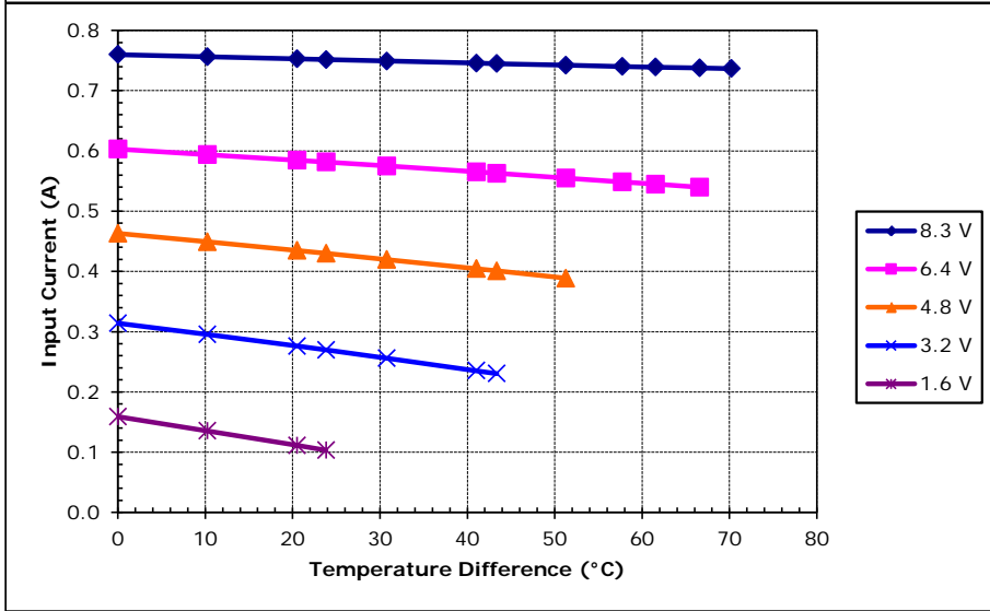
Unpotted TE-66-0.45-1.3 at a hot-side temperature of 30 °C
