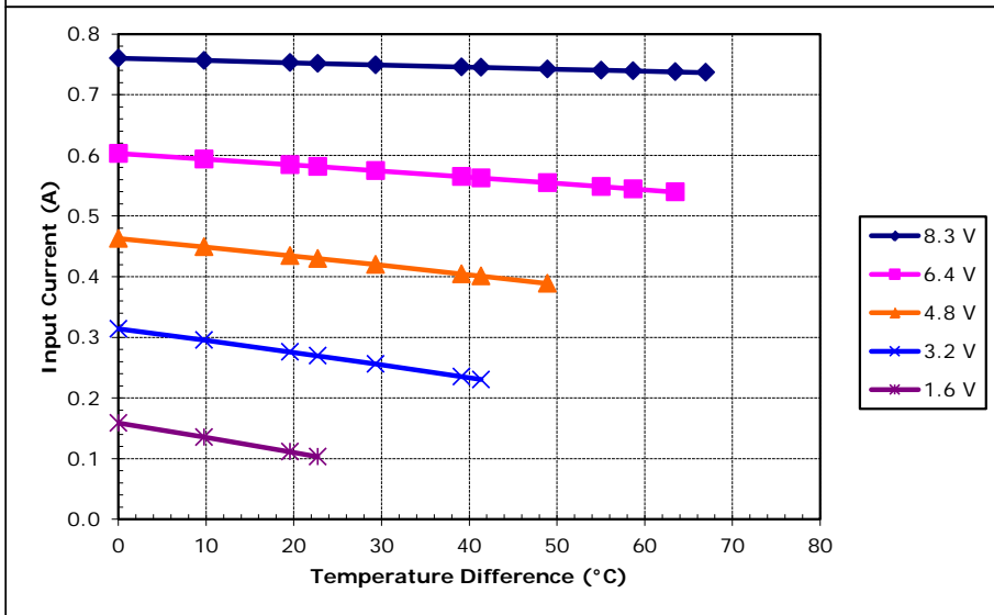
Potted TE-66-0.45-1.3 at a hot-side temperature of 30 °C
