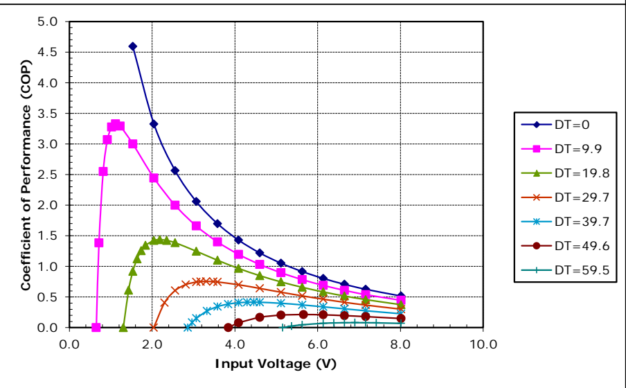
Potted TE-65-0.6-1.5 at a hot-side temperature of 30 °C
