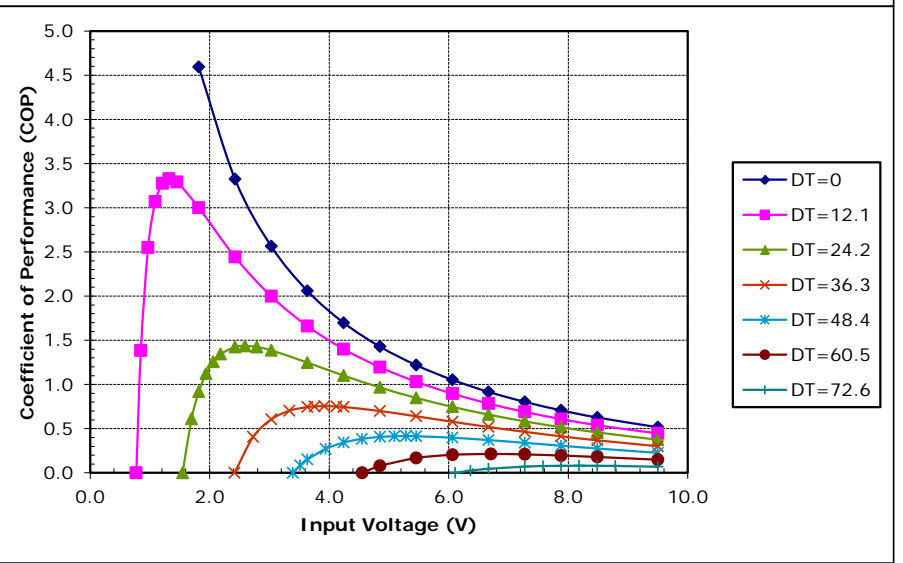
Potted TE-65-0.6-1.5 at a hot-side temperature of 70 °C
