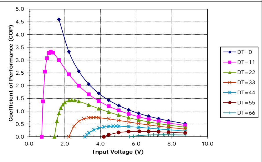
Potted TE-65-0.6-1.5 at a hot-side temperature of 50 °C
