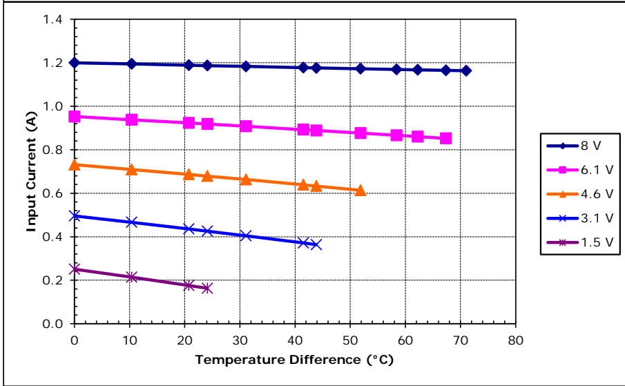
Unpotted TE-65-0.6-1.5 at a hot-side temperature of 30 °C
