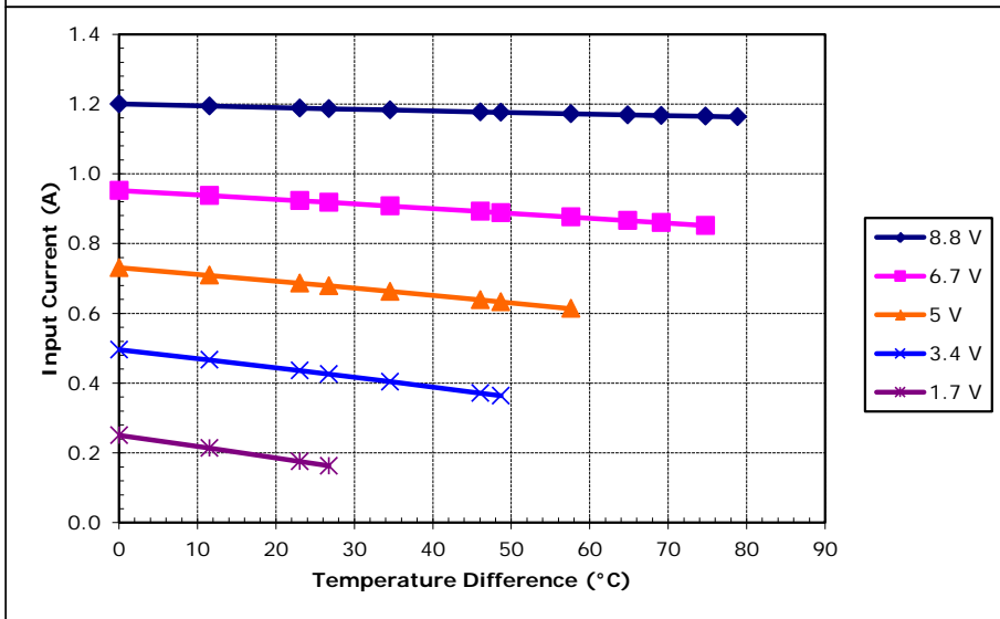
Unpotted TE-65-0.6-1.5 at a hot-side temperature of 50 °C
