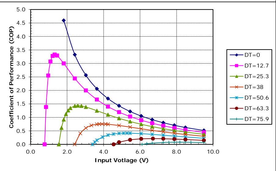
Unpotted TE-65-0.6-1.5 at a hot-side temperature of 70 °C
