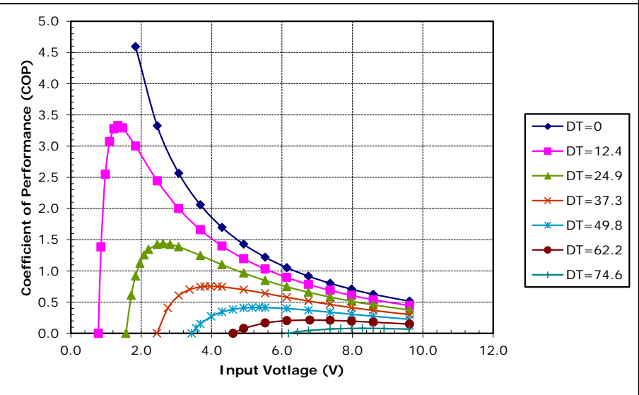
Unpotted TE-65-0.6-1.2 at a hot-side temperature of 70 °C
