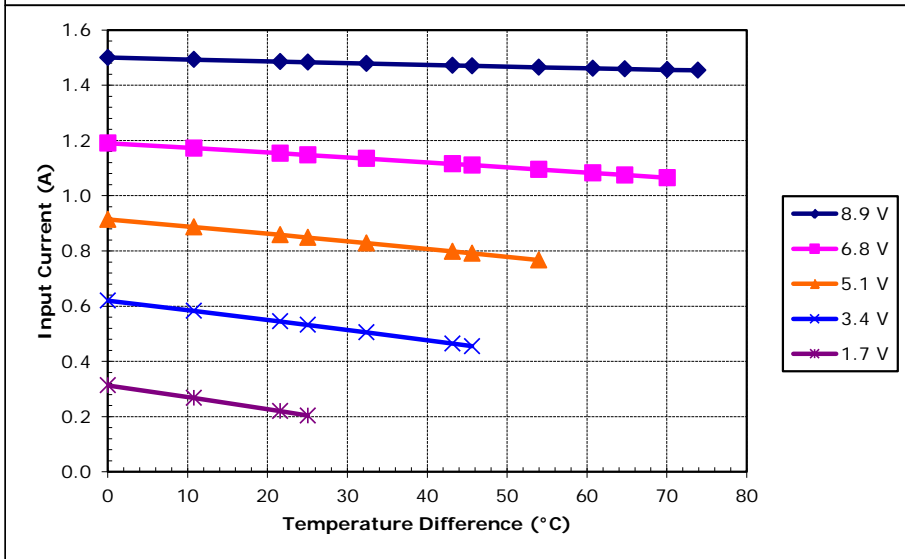
Potted TE-65-0.6-1.2 at a hot-side temperature of 50 °C
