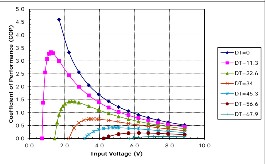
Unpotted TE-65-0.6-1.2 at a hot-side temperature of 50 °C
