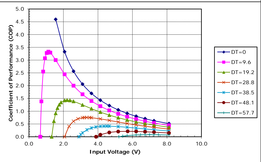
Potted TE-65-0.6-0.8 at a hot-side temperature of 30 °C
