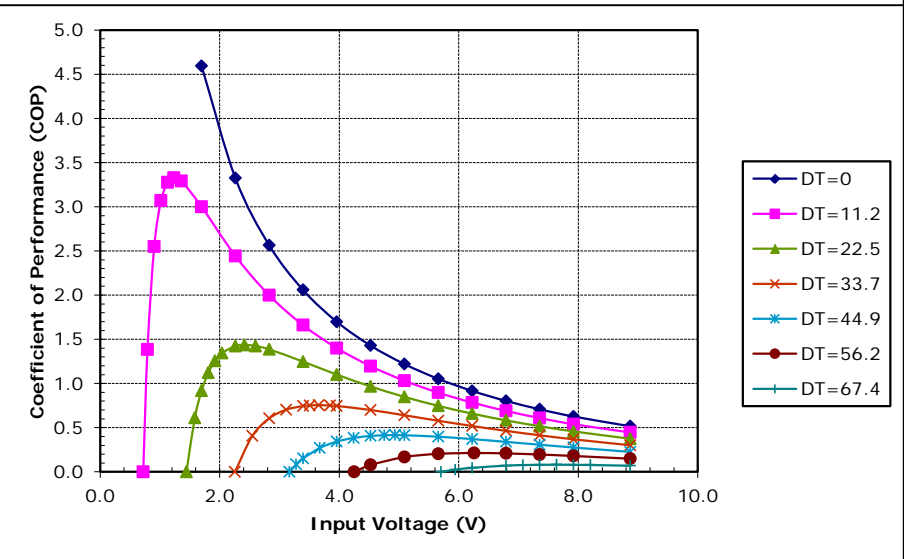
Unpotted TE-65-0.6-0.8 at a hot-side temperature of 50 °C
