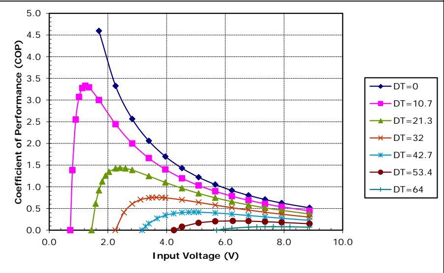
Potted TE-65-0.6-0.8 at a hot-side temperature of 50 °C
