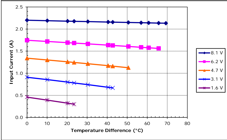
Unpotted TE-65-0.6-0.8 at a hot-side temperature of 30 °C
