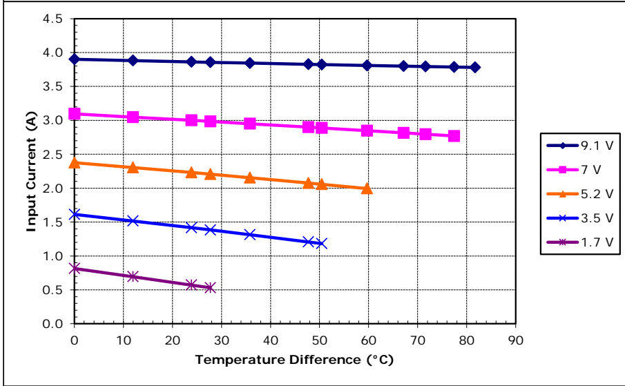
Potted TE-63-1.4-2.5 at a hot-side temperature of 70 °C
