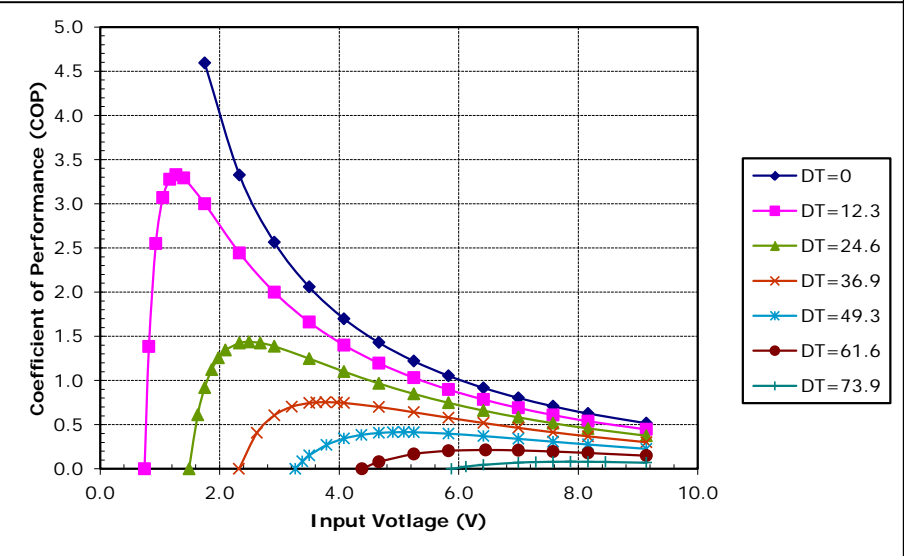
Unpotted TE-63-1.4-1.5 at a hot-side temperature of 70 °C
