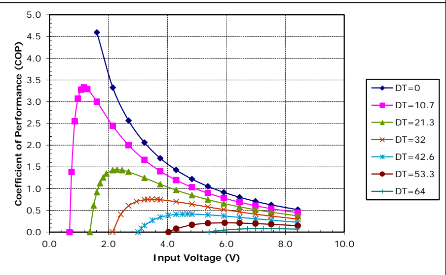
Potted TE-63-1.4-1.5 at a hot-side temperature of 50 °C
