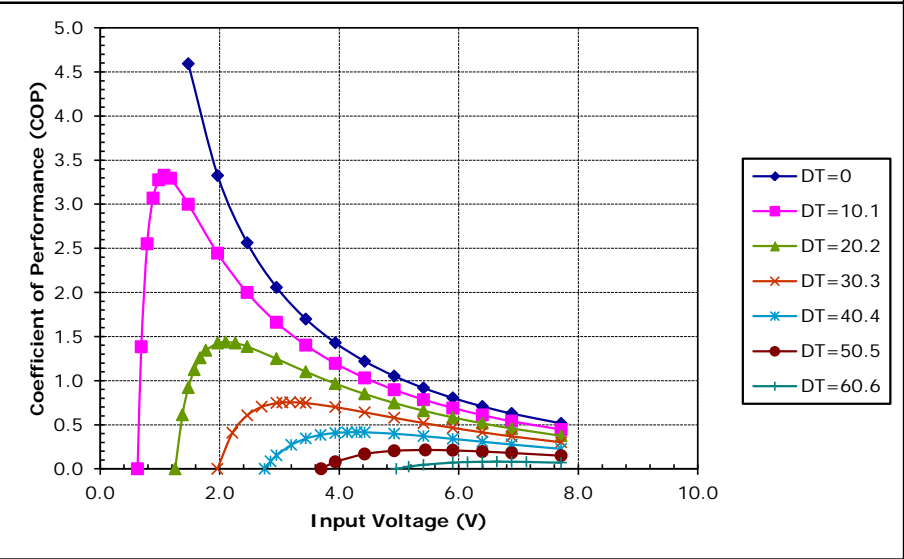
Unpotted TE-63-1.4-1.5 at a hot-side temperature of 30 °C
