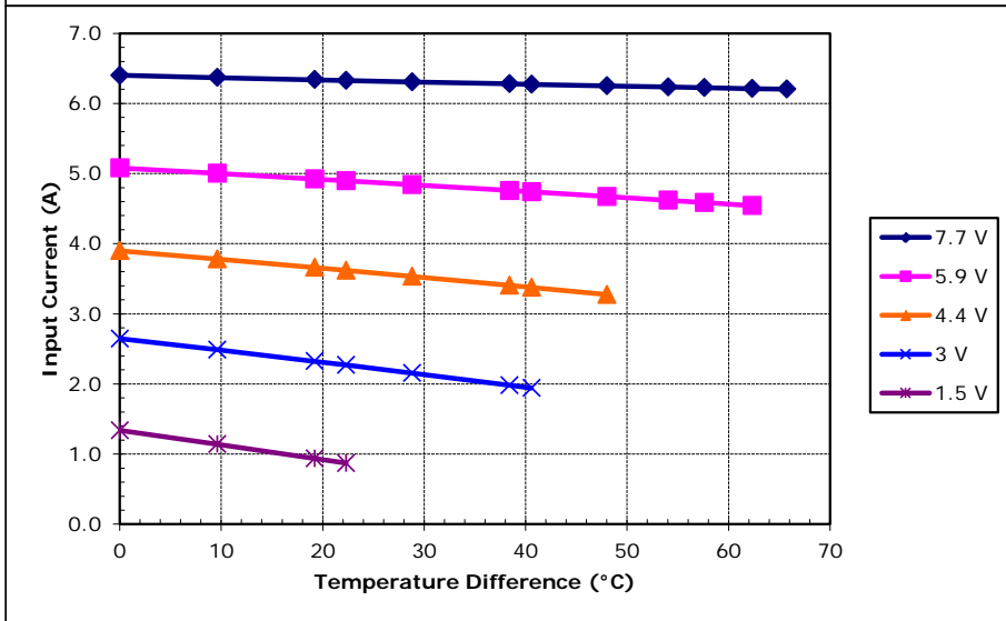
Potted TE-63-1.4-1.5 at a hot-side temperature of 30 °C
