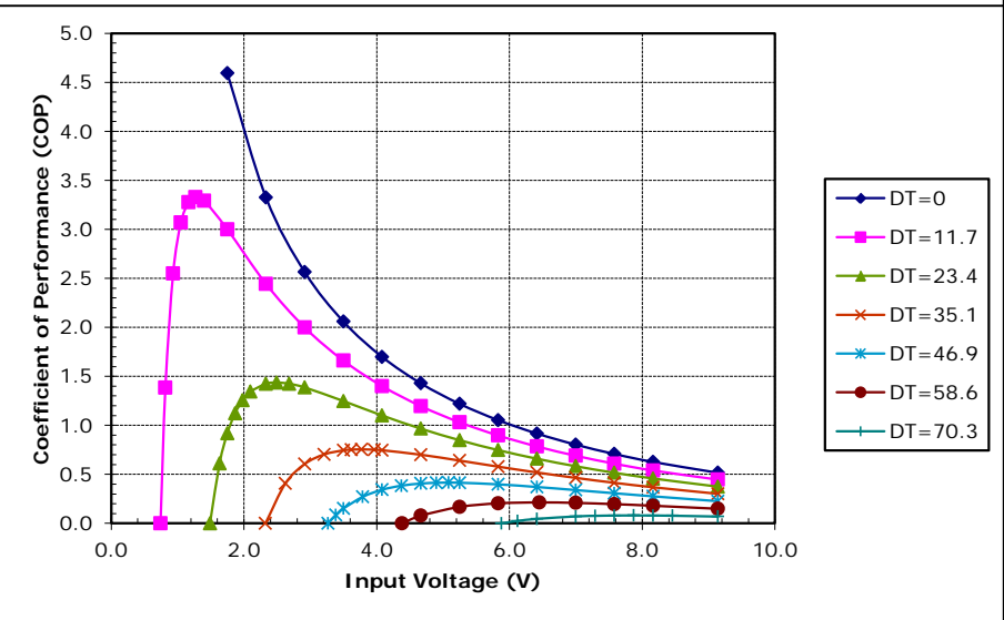
Potted TE-63-1.4-1.5 at a hot-side temperature of 70 °C
