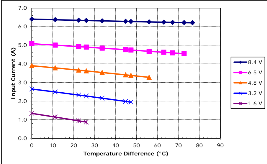
Unpotted TE-63-1.4-1.5 at a hot-side temperature of 50 °C
