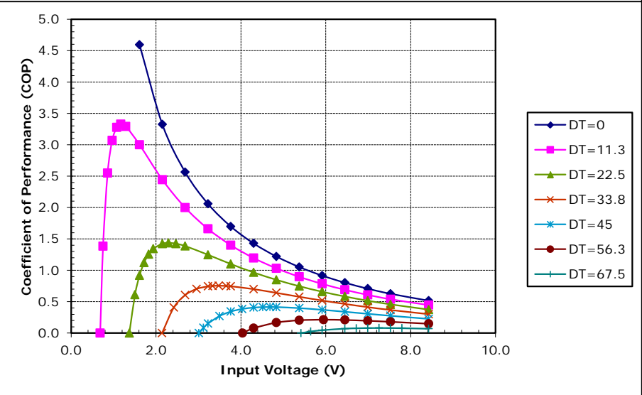
Unpotted TE-63-1.0-1.5 at a hot-side temperature of 50 °C
