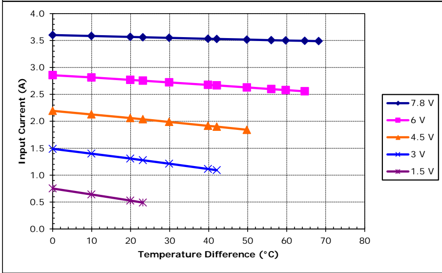
Unpotted TE-63-1.0-1.3 at a hot-side temperature of 30 °C
