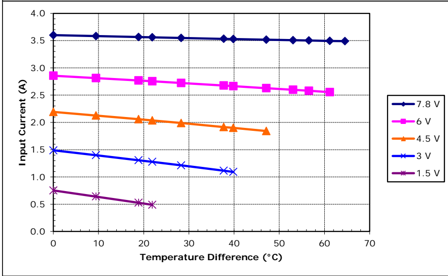
Potted TE-63-1.0-1.3 at a hot-side temperature of 30 °C
