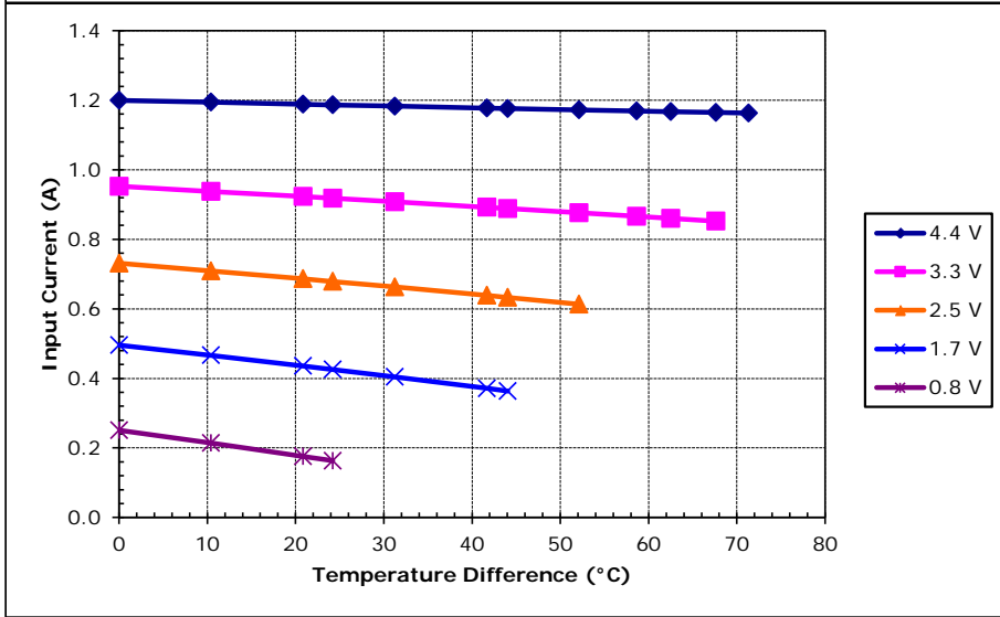
Unpotted TE-35-0.6-1.5 at a hot-side temperature of 30 °C
