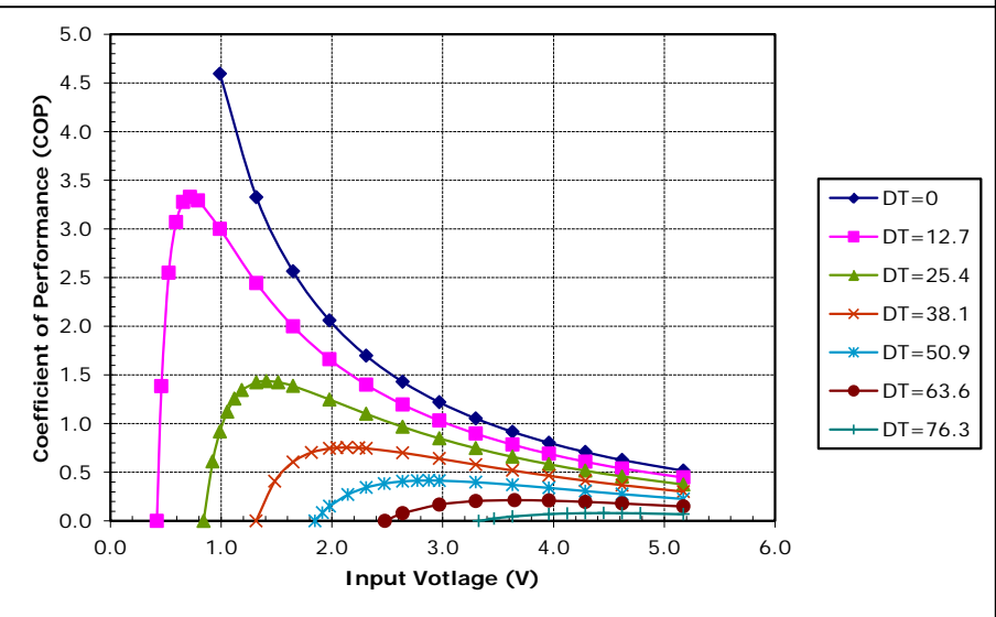
Unpotted TE-35-0.6-1.5 at a hot-side temperature of 70 °C
