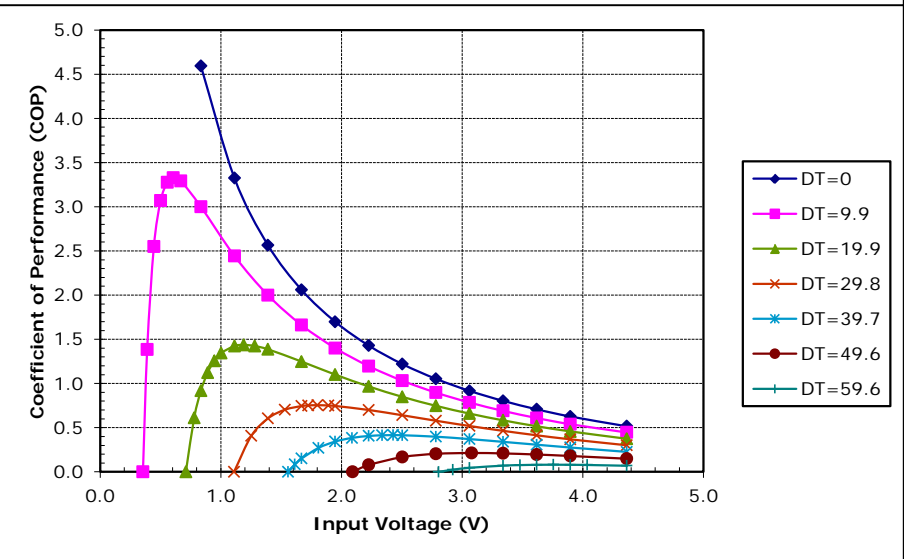
Potted TE-35-0.6-1.5 at a hot-side temperature of 30 °C
