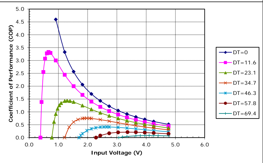
Unpotted TE-35-0.6-1.5 at a hot-side temperature of 50 °C
