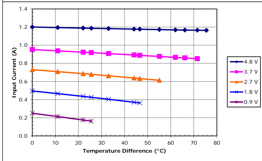
Potted TE-35-0.6-1.5 at a hot-side temperature of 50 °C
