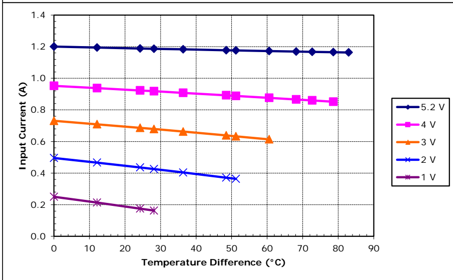
Potted TE-35-0.6-1.5 at a hot-side temperature of 70 °C
