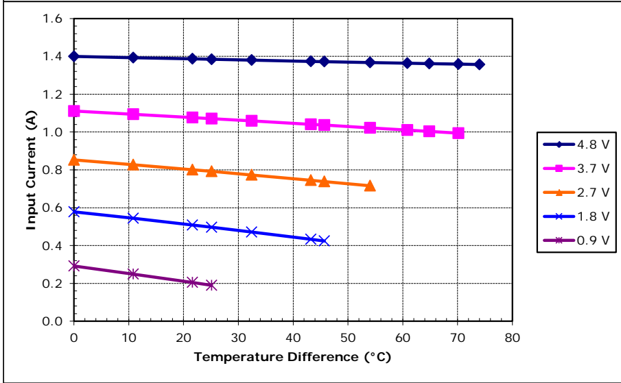
Potted TE-35-0.6-1.2 at a hot-side temperature of 50 °C
