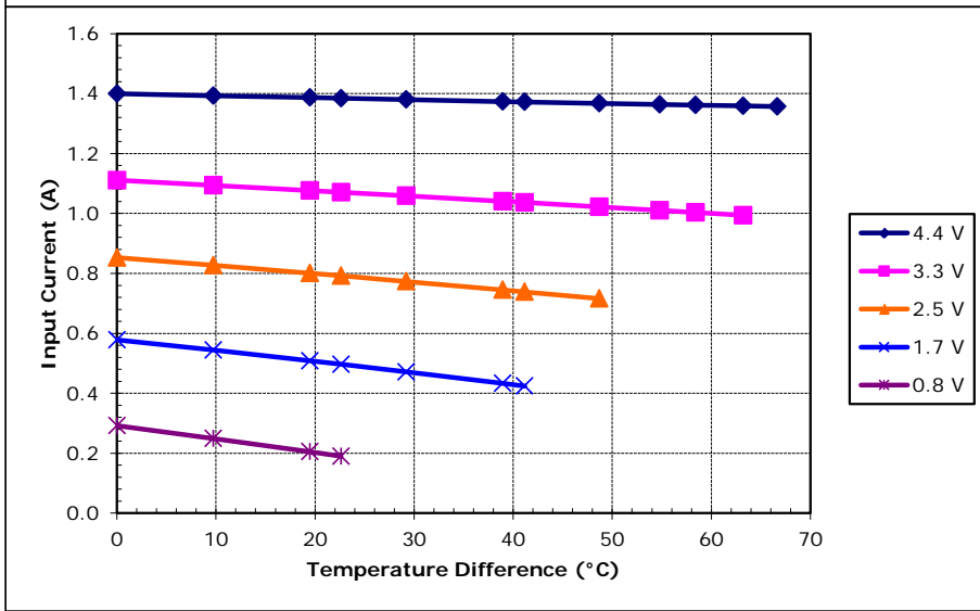
Potted TE-35-0.6-1.2 at a hot-side temperature of 30 °C
