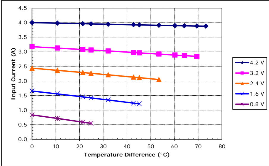
Potted TE-31-1.4-2.5 at a hot-side temperature of 50 °C
