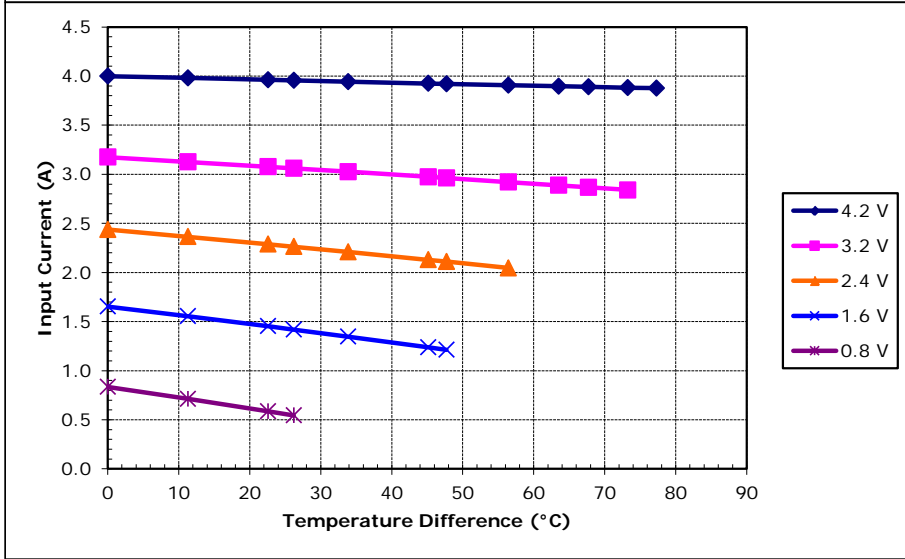
Unpotted TE-31-1.4-2.5 at a hot-side temperature of 50 °C
