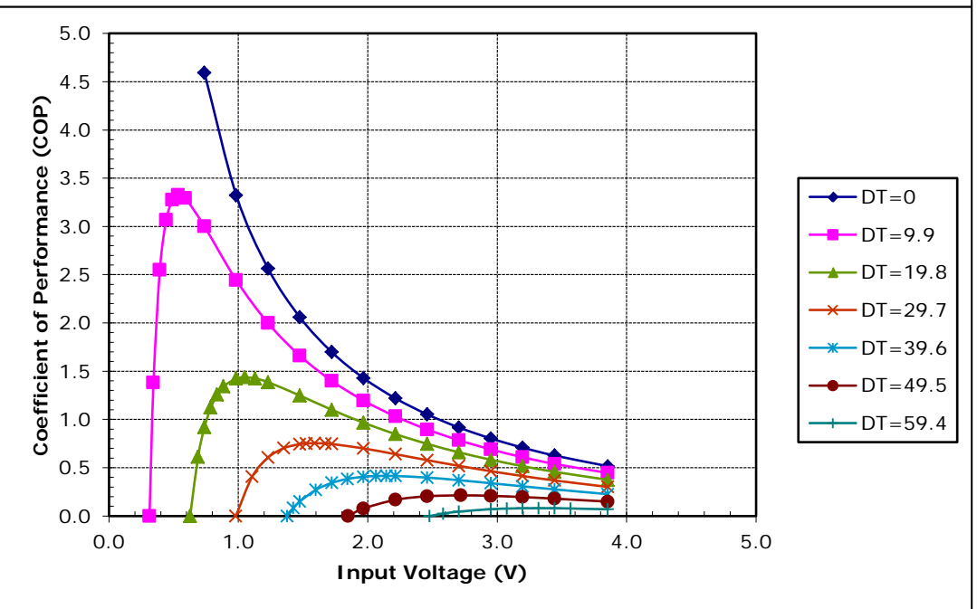
Potted TE-31-0.6-1.5 at a hot-side temperature of 30 °C
