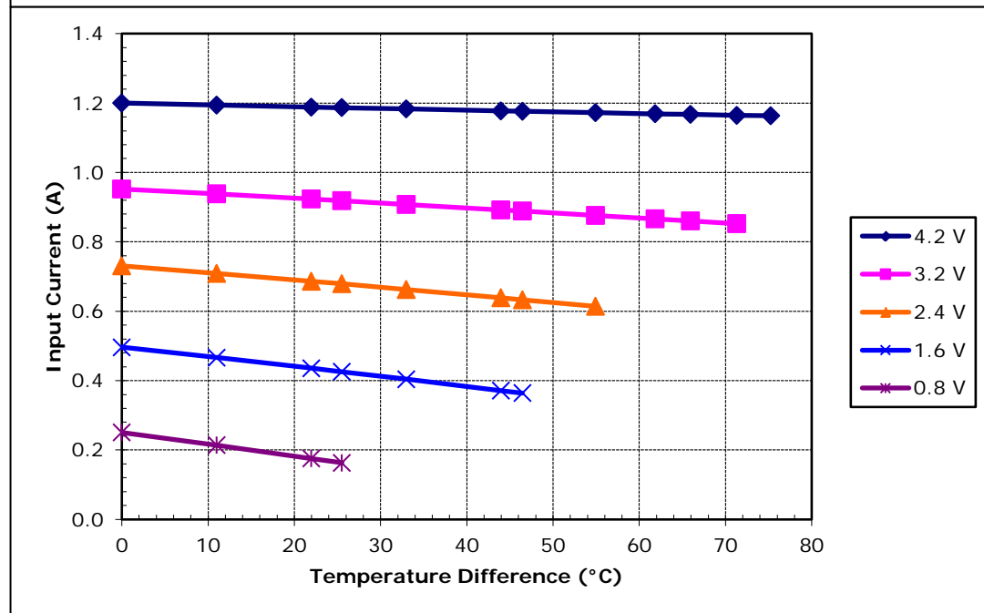
Potted TE-31-0.6-1.5 at a hot-side temperature of 50 °C
