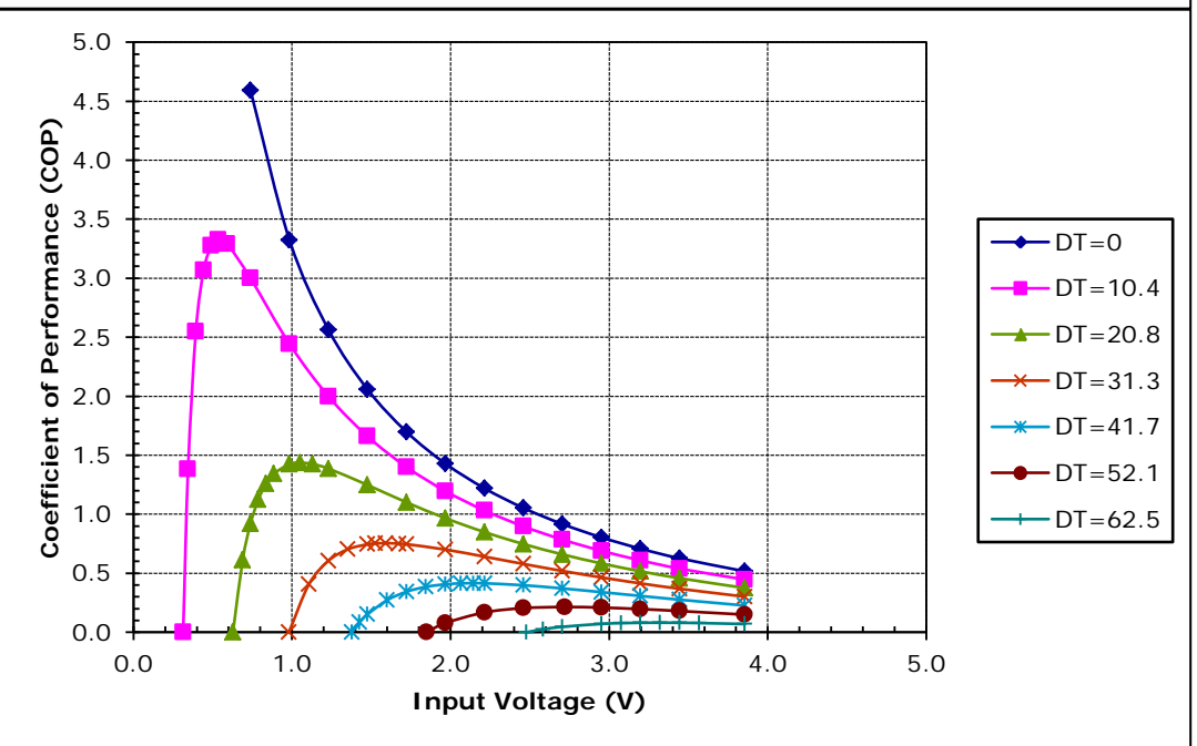
Unpotted TE-31-0.6-1.5 at a hot-side temperature of 30 °C
