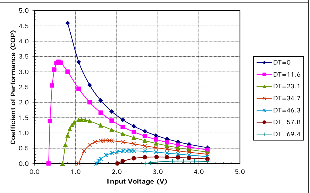
Unpotted TE-31-0.6-1.5 at a hot-side temperature of 50 °C
