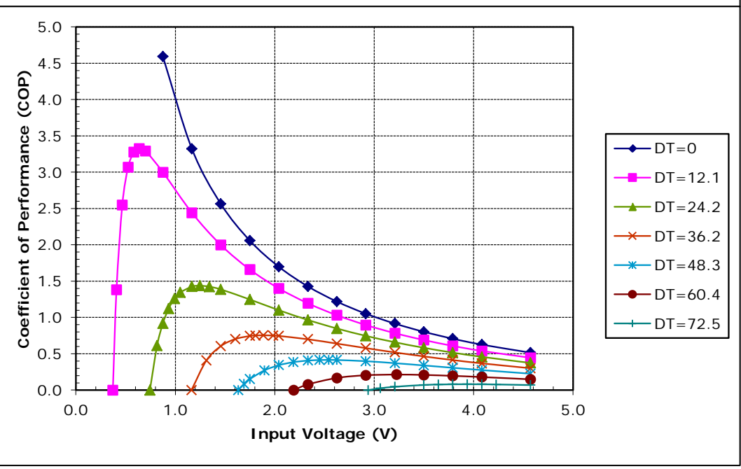
Potted TE-31-0.6-1.5 at a hot-side temperature of 70 °C
