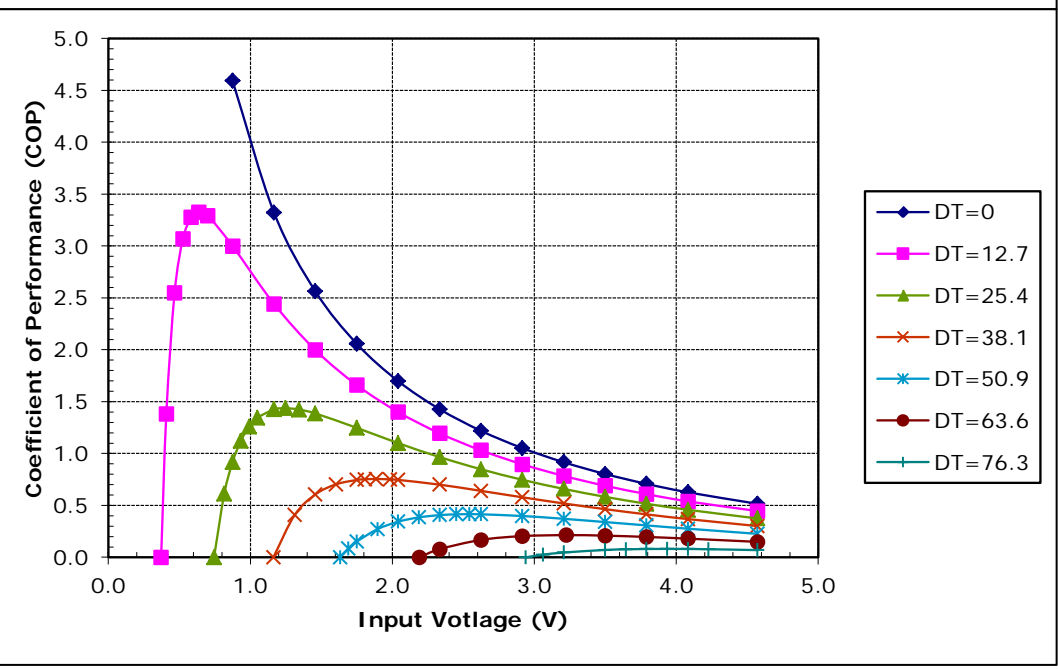
Unpotted TE-31-0.6-1.5 at a hot-side temperature of 70 °C
