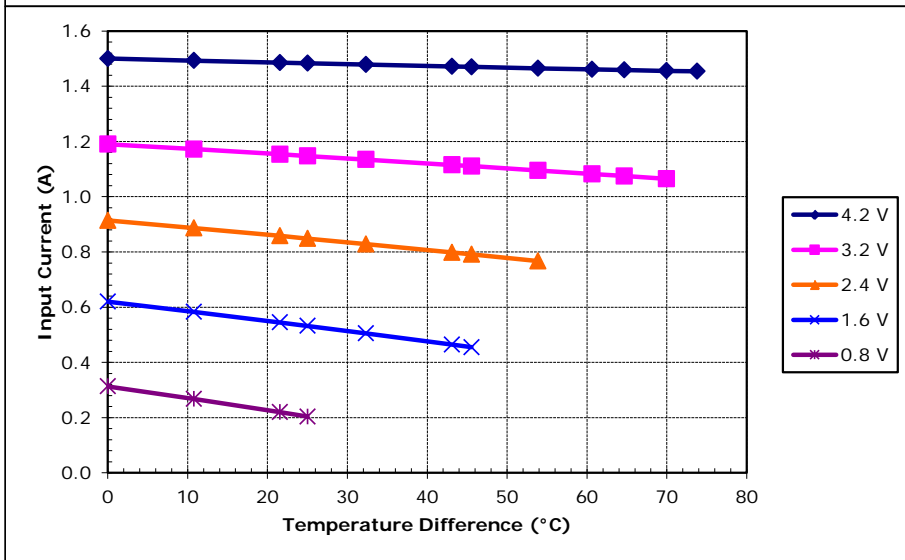
Potted TE-31-0.6-1.2 at a hot-side temperature of 50 °C
