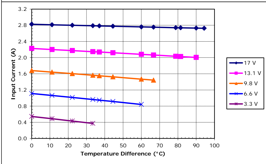
Potted TE-2-(127-127)-1.3 at a hot-side temperature of 50 °C
