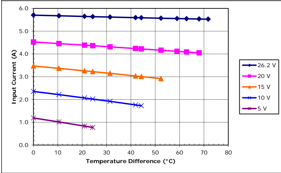
Potted TE-195-1.0-0.8 at a hot-side temperature of 50 °C
