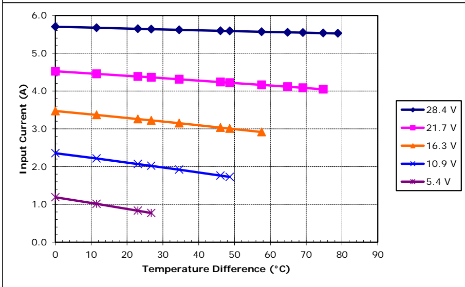
Potted TE-195-1.0-0.8 at a hot-side temperature of 70 °C
