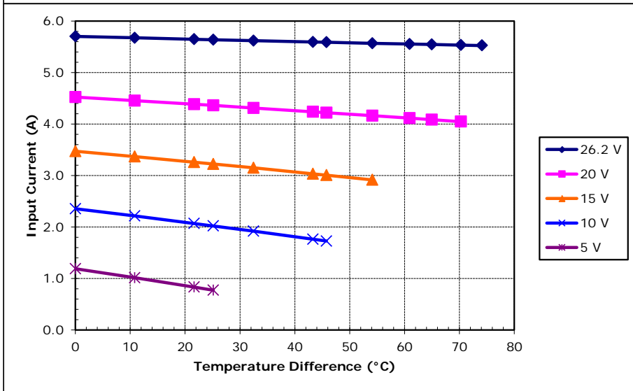
Unpotted TE-195-1.0-0.8 at a hot-side temperature of 50 °C
