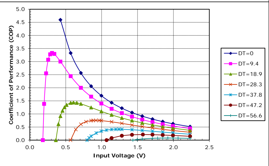
Potted TE-18-0.45-1.3 at a hot-side temperature of 30 °C
