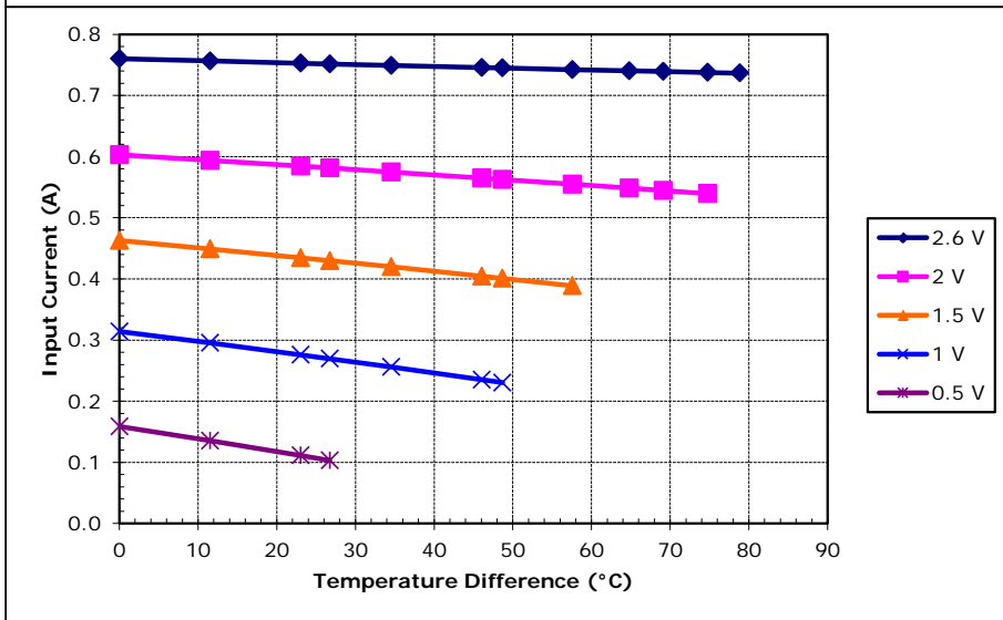
Potted TE-18-0.45-1.3 at a hot-side temperature of 70 °C
