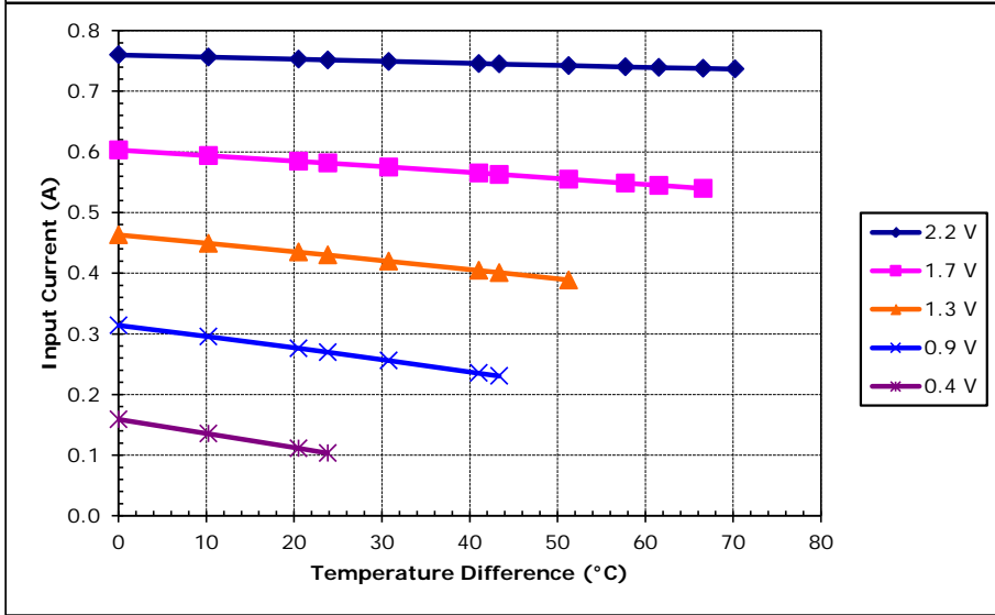
Unpotted TE-18-0.45-1.3 at a hot-side temperature of 30 °C
