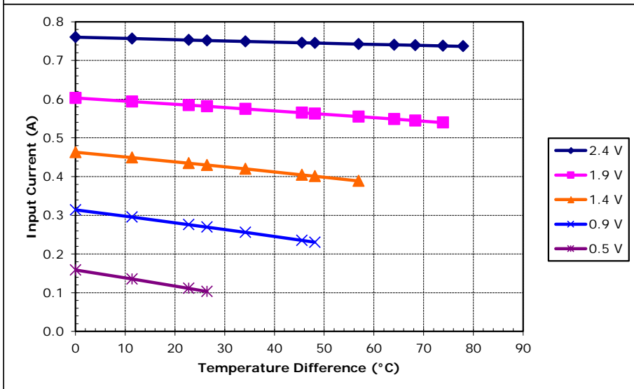
Unpotted TE-18-0.45-1.3 at a hot-side temperature of 50 °C
