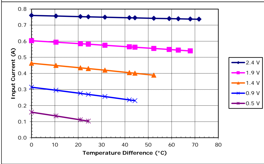
Potted TE-18-0.45-1.3 at a hot-side temperature of 50 °C
