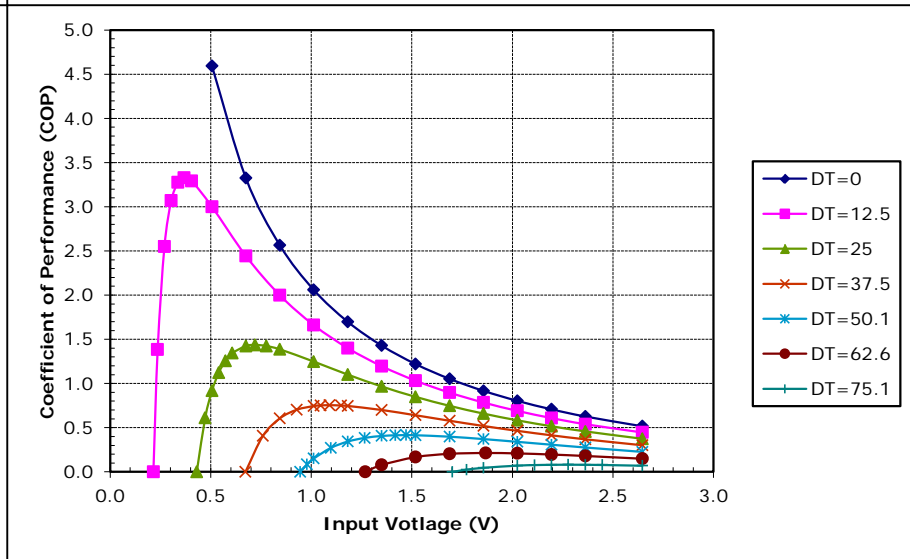
Unpotted TE-18-0.45-1.3 at a hot-side temperature of 70 °C
