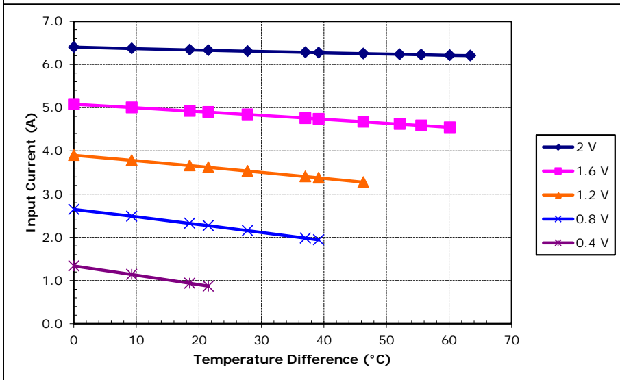
Potted TE-17-1.4-1.5 at a hot-side temperature of 30 °C
