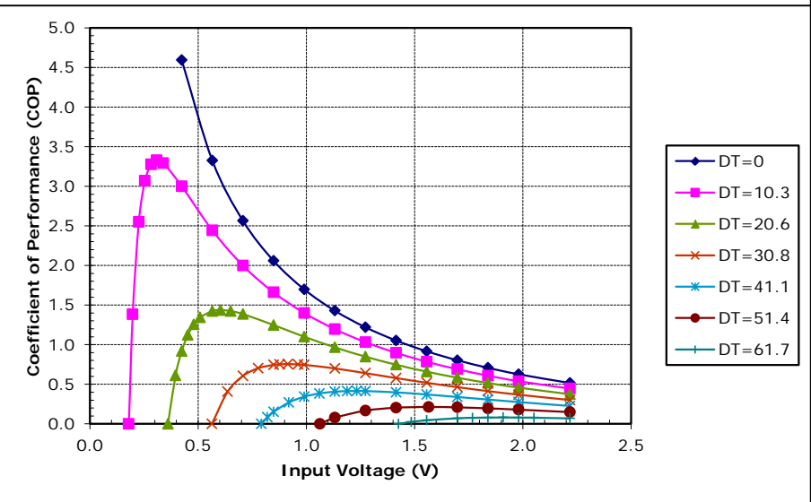
Potted TE-17-1.4-1.5 at a hot-side temperature of 50 °C
