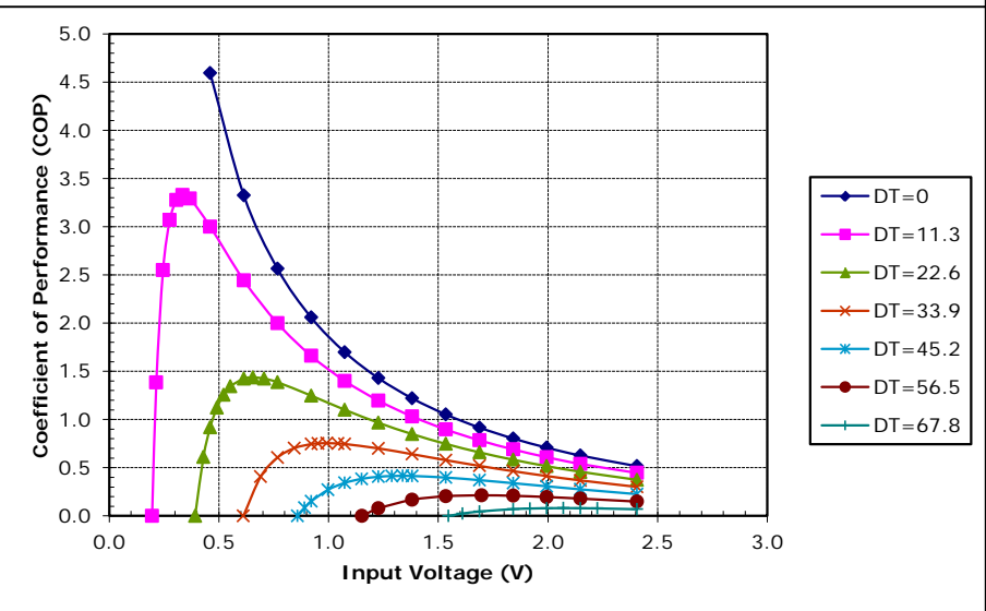
Potted TE-17-1.4-1.5 at a hot-side temperature of 70 °C
