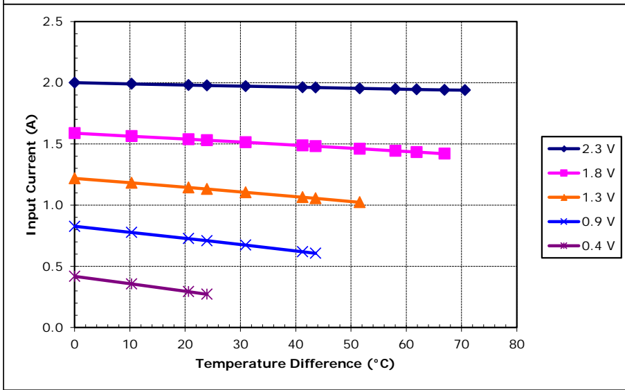
Potted TE-17-1.0-2.5 at a hot-side temperature of 50 °C
