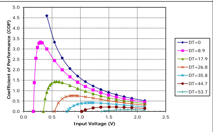
Potted TE-17-1.0-1.3 at a hot-side temperature of 30 °C
