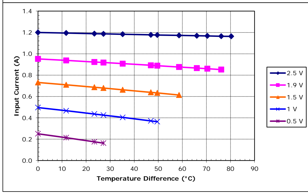
Potted TE-17-0.6-1.5 at a hot-side temperature of 70 °C
