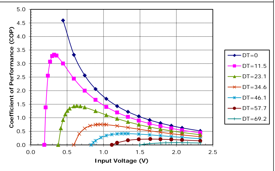
Unpotted TE-17-0.6-1.5 at a hot-side temperature of 50 °C
