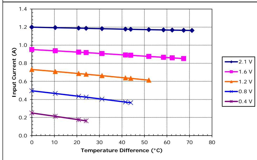
Unpotted TE-17-0.6-1.5 at a hot-side temperature of 30 °C
