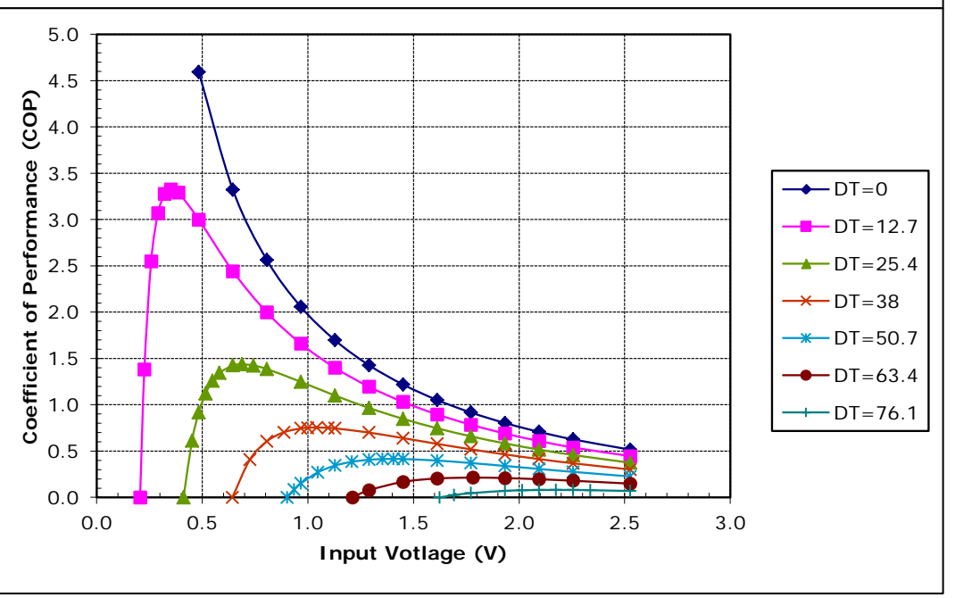
Unpotted TE-17-0.6-1.5 at a hot-side temperature of 70 °C
