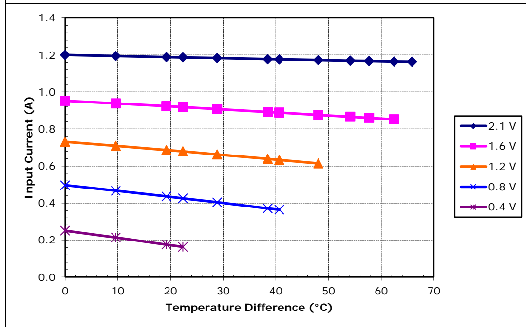
Potted TE-17-0.6-1.5 at a hot-side temperature of 30 °C
