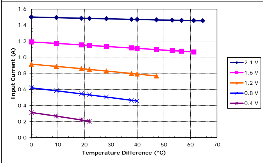
Potted TE-17-0.6-1.2 at a hot-side temperature of 30 °C
