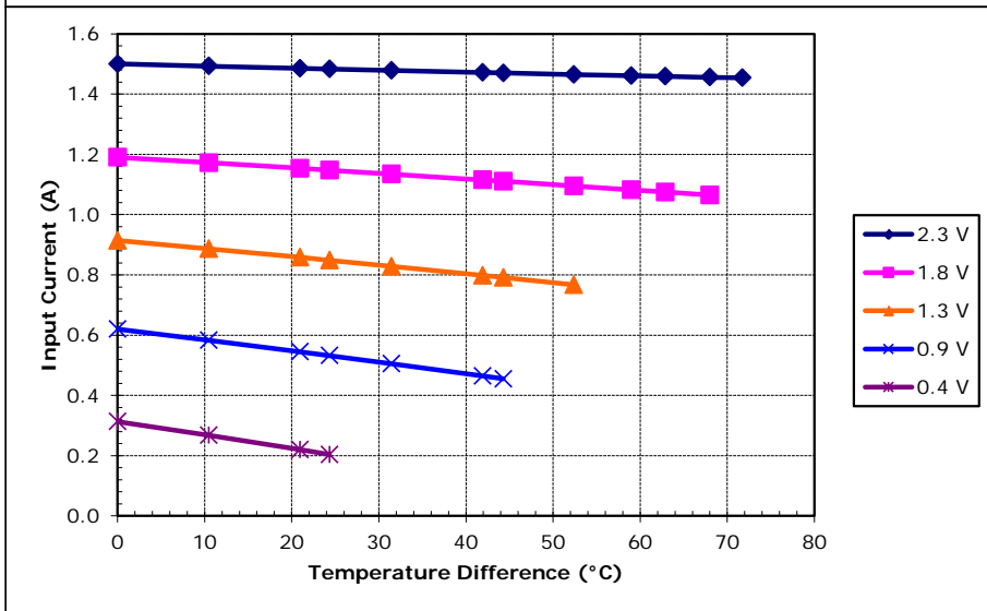
Potted TE-17-0.6-1.2 at a hot-side temperature of 50 °C
