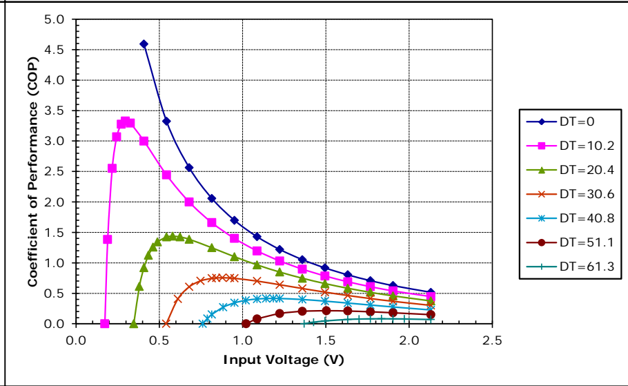
Unpotted TE-17-0.6-1.2 at a hot-side temperature of 30 °C
