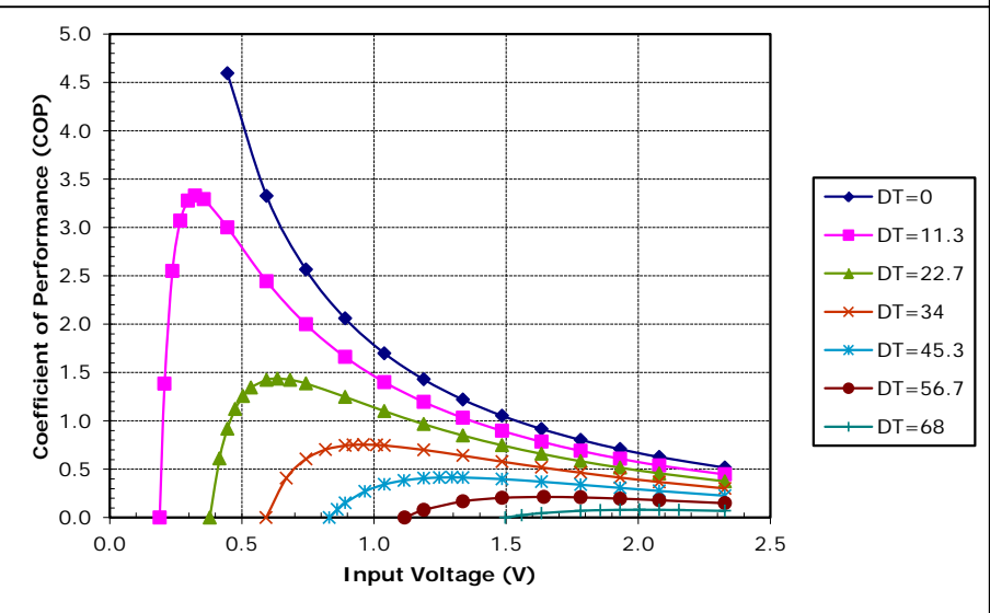
Unpotted TE-17-0.6-1.2 at a hot-side temperature of 50 °C
