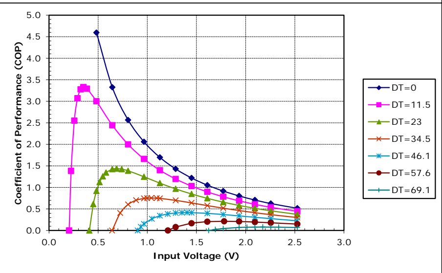
Potted TE-17-0.6-1.2 at a hot-side temperature of 70 °C
