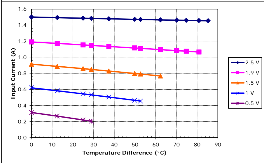
Unpotted TE-17-0.6-1.2 at a hot-side temperature of 70 °C
