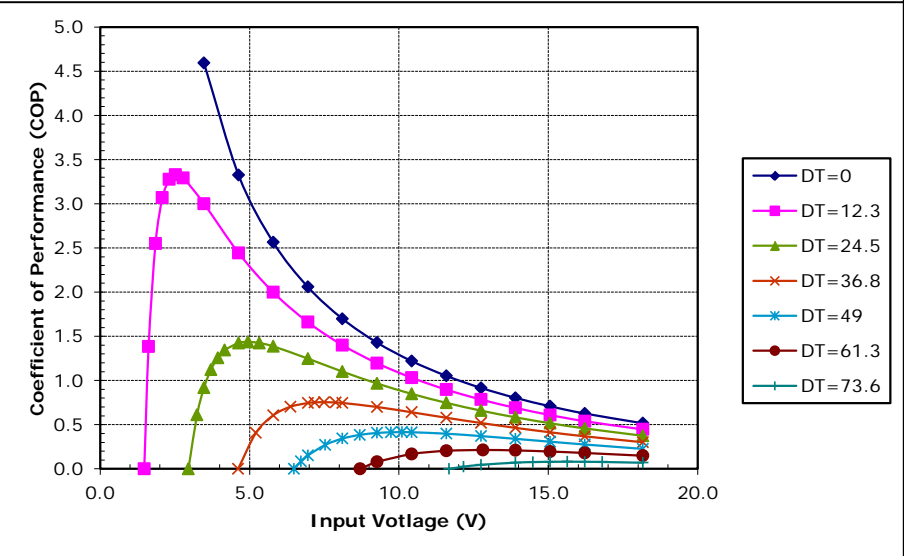
Unpotted TE-127-2.0-1.5 at a hot-side temperature of 70 °C
