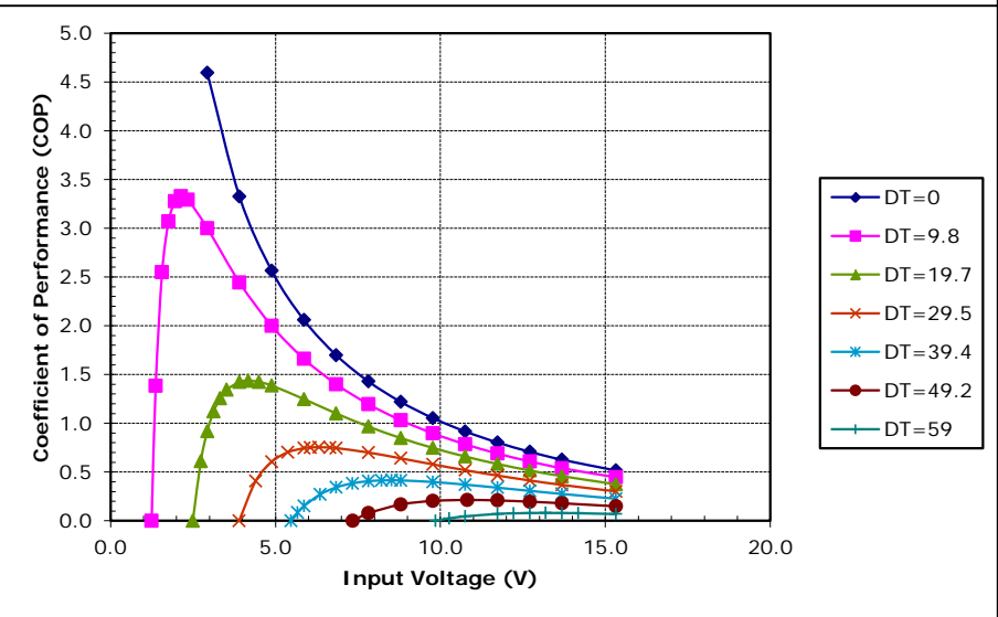
Potted TE-127-2.0-1.5 at a hot-side temperature of 30 °C
