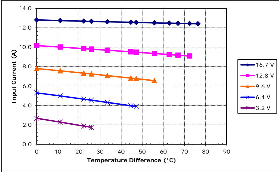
Unpotted TE-127-2.0-1.5 at a hot-side temperature of 50 °C
