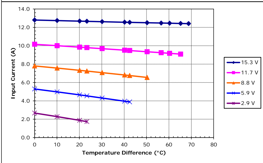
Unpotted TE-127-2.0-1.5 at a hot-side temperature of 30 °C
