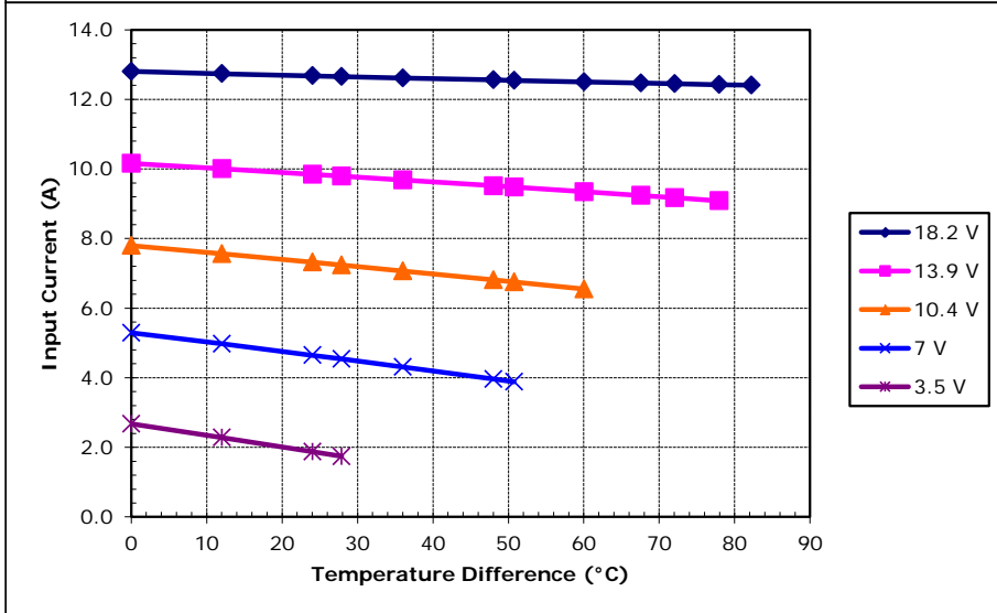
Potted TE-127-2.0-1.5 at a hot-side temperature of 70 °C
