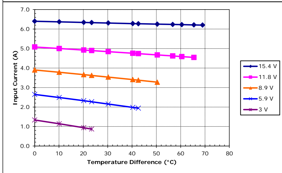
Unpotted TE-127-1.4-1.5 at a hot-side temperature of 30 °C
