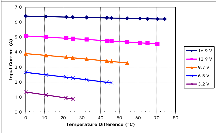
Potted TE-127-1.4-1.5 at a hot-side temperature of 50 °C
