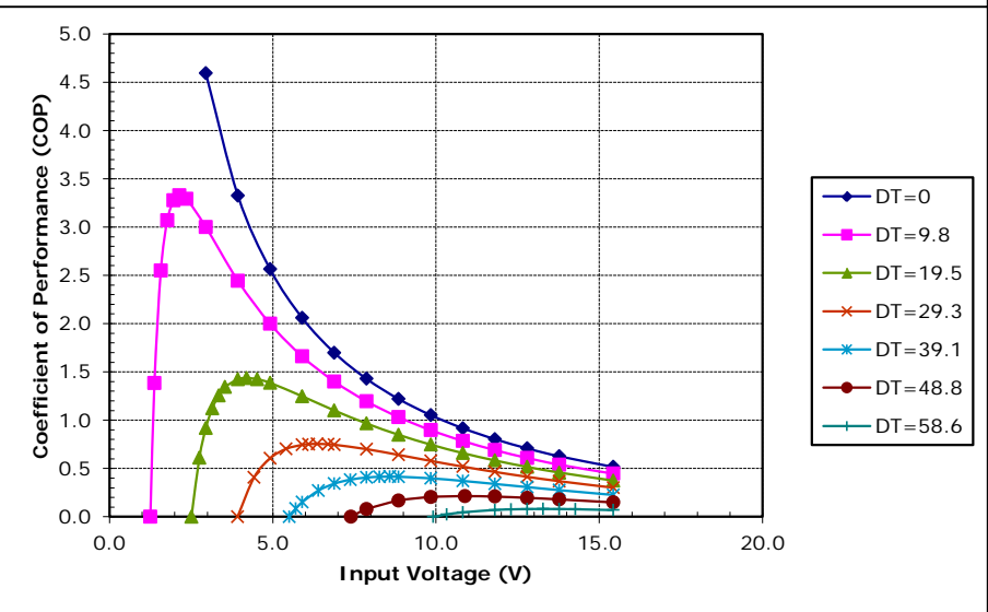
Potted TE-127-1.4-1.5 at a hot-side temperature of 30 °C
