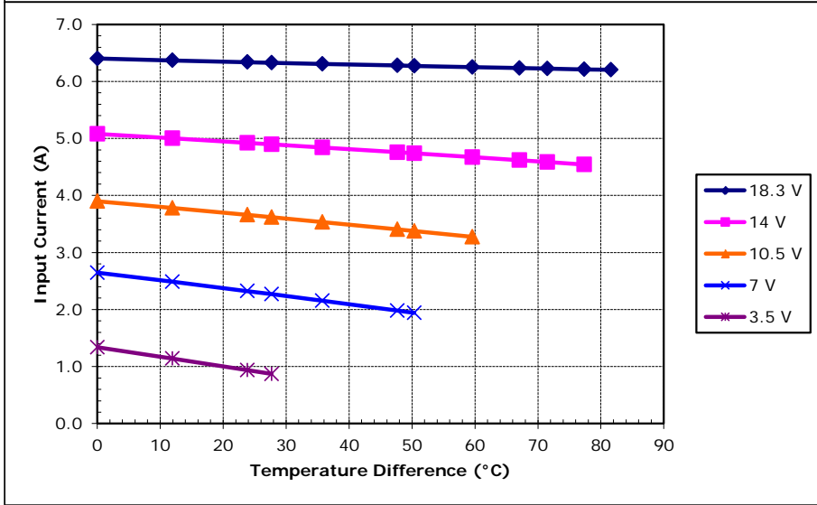
Potted TE-127-1.4-1.5 at a hot-side temperature of 70 °C
