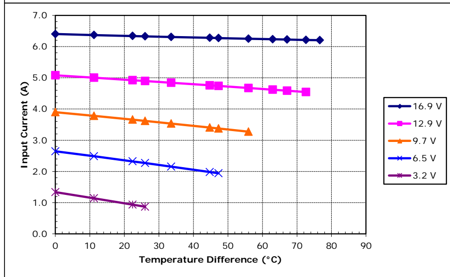
Unpotted TE-127-1.4-1.5 at a hot-side temperature of 50 °C
