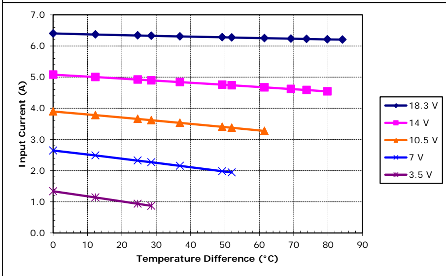
Unpotted TE-127-1.4-1.5 at a hot-side temperature of 70 °C
