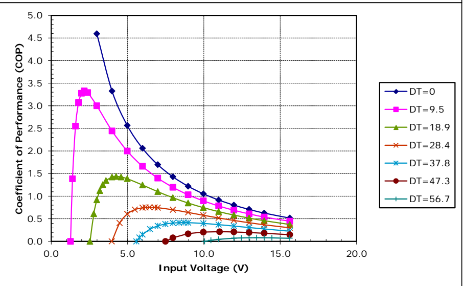
Potted TE-127-1.4-1.15 at a hot-side temperature of 30 °C
