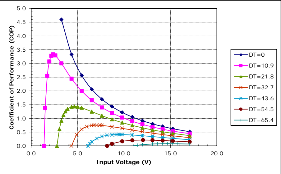
Unpotted TE-127-1.4-1.15 at a hot-side temperature of 50 °C
