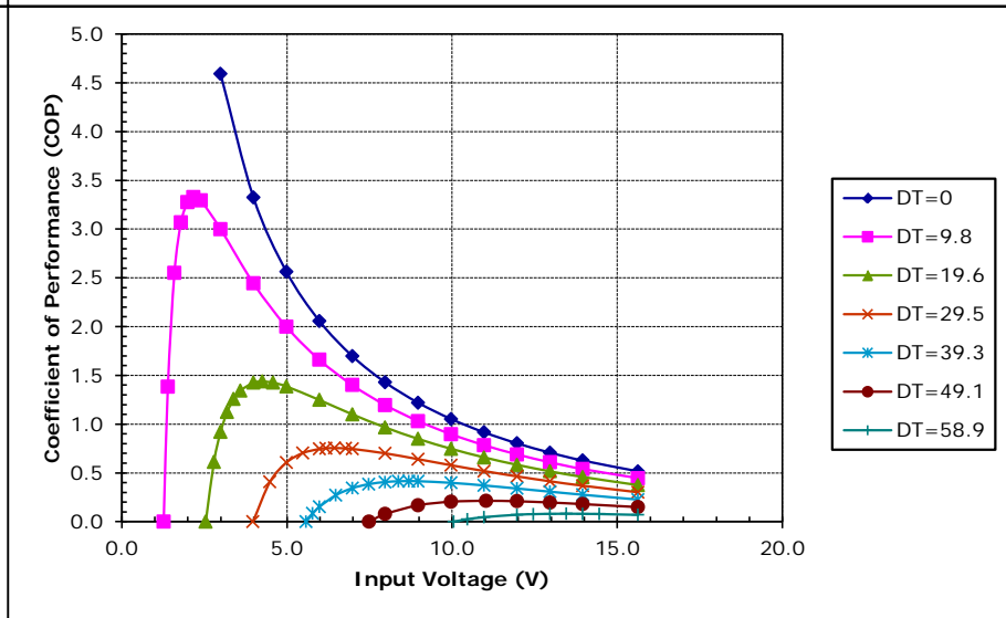
Unpotted TE-127-1.4-1.15 at a hot-side temperature of 30 °C
