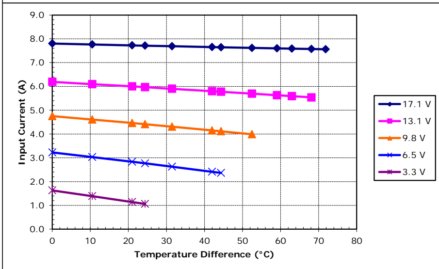
Potted TE-127-1.4-1.15 at a hot-side temperature of 50 °C
