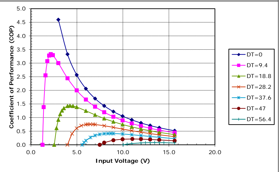
Potted TE-127-1.4-1.05 at a hot-side temperature of 30 °C
