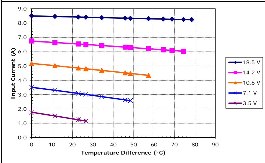
Potted TE-127-1.4-1.05 at a hot-side temperature of 70 °C
