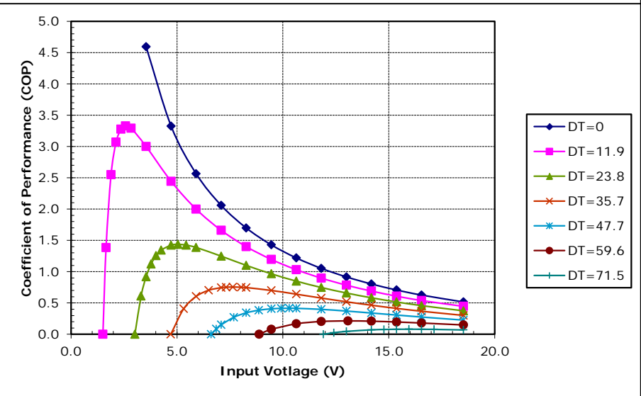
Unpotted TE-127-1.4-1.05 at a hot-side temperature of 70 °C
