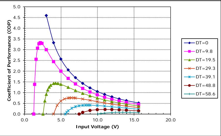
Unpotted TE-127-1.4-1.05 at a hot-side temperature of 30 °C
