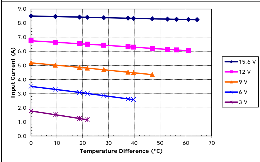
Potted TE-127-1.4-1.05 at a hot-side temperature of 30 °C
