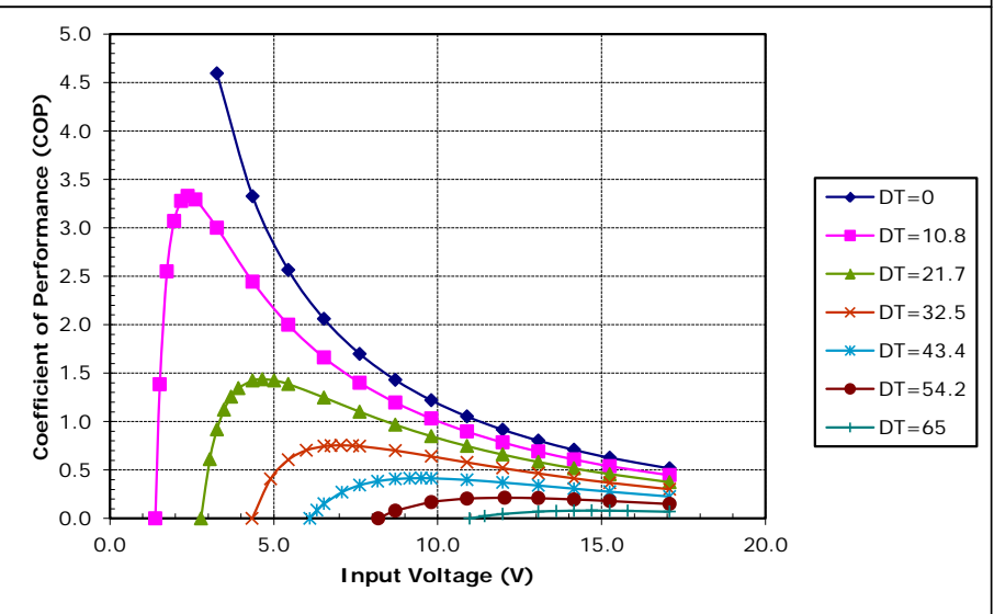
Unpotted TE-127-1.4-1.05 at a hot-side temperature of 50 °C
