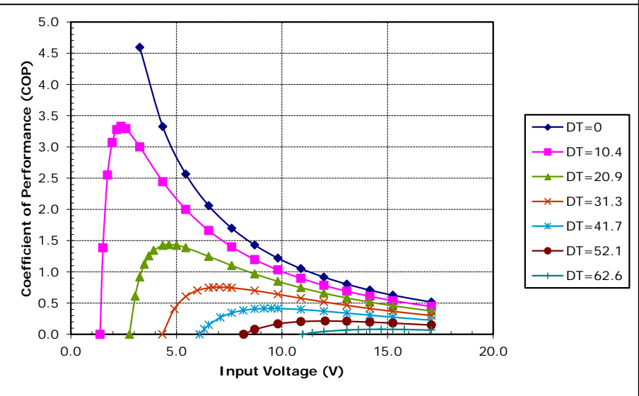
Potted TE-127-1.4-1.05 at a hot-side temperature of 50 °C
