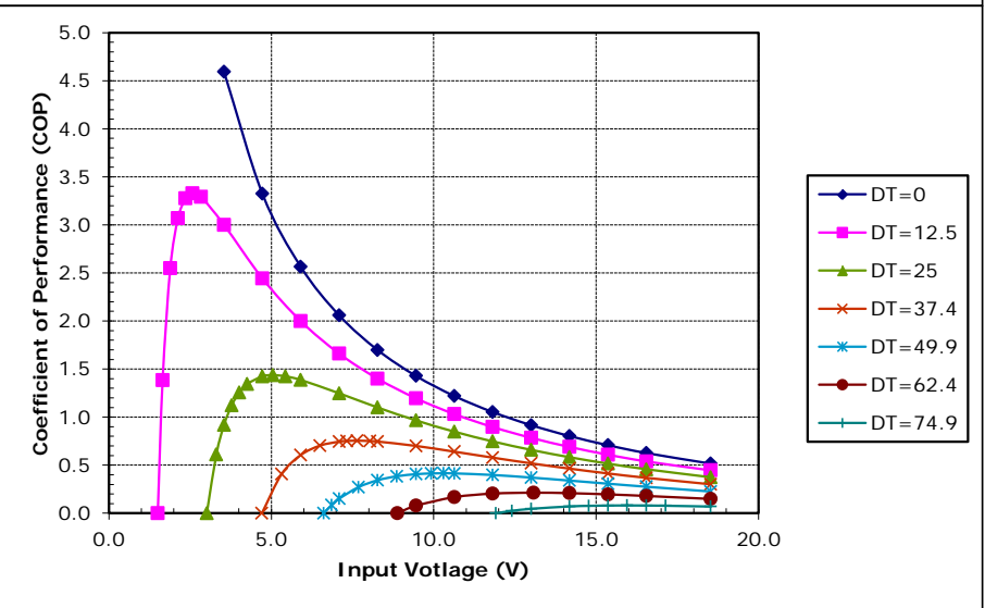
Unpotted TE-127-1.0-2.5 at a hot-side temperature of 70 °C
