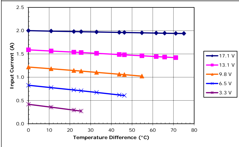
Potted TE-127-1.0-2.5 at a hot-side temperature of 50 °C
